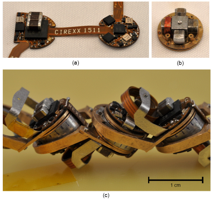
Fig. 7. Milli-Motein Detail Views. (a) The repeating section of the Milli-Motein flex circuit. The processor board (left) contains an 8-bit microcontroller, a capacitor bank to store pulse power for the actuator, and one of the three half-bridge motor drivers. The motor driver board (right) contains the other two half-bridge motor drivers and two-axis magnetoresistive sensor at the center. (b) Partially assembled electropermanent motor. Only one of the four coils are installed in this photo. The stator core and the tips of the stator arms are made of iron. Each arm is interrupted by a parallel pair of NdFeB and Alnico magnets, forming a switchable electropermanent magnet. A ball thrust bearing and motor-driver-side bushing are also visible in this photo. (c) Fully assembled Milli-Motein.
