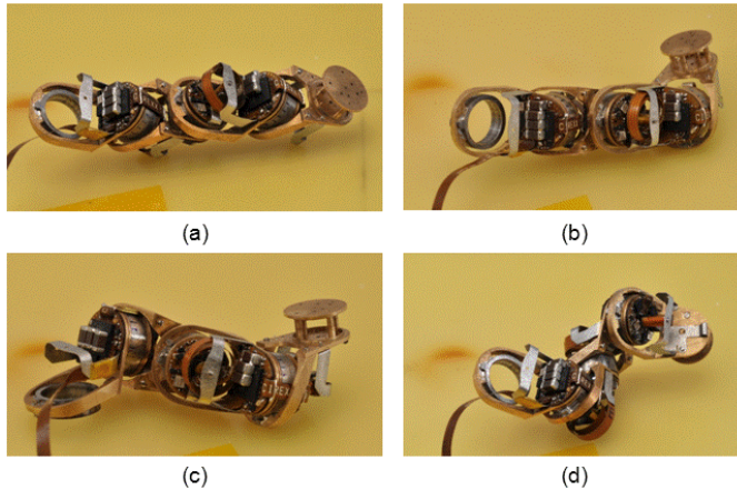
Fig. 9. Four-segment Milli-Motein rendering four geometric shapes. (a) straight line [0\ 0\ 0] (b) L-shape [0\ 0\ 90] (c) periscope [-90\ 0\ 90] (d) helix. [90\ 90\ 90]
