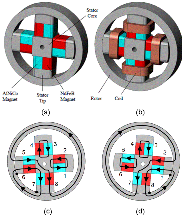
Fig. 4. Electropermanent Wobble Stepper Motor. Electropermanent stepper motor principle of operation. The red magnets are NdFeB, always polarized in the direction shown. The magnetization of the blue Alnico magnets switches as the motor operates. The motor starts in position (c), with magnets 5-6 and 7-8 on, and magnets 1-2 and 3-4 off. Flux flows through the rotor and stator as shown. Applying a current pulse to the horizontal winding around magnets 5-6 and 2-1 switches the magnetization of magnets 5 and 1, turning magnet 5-6 off and magnet 2-1 on, resulting in the new flux paths shown at right. The rotor pivots counterclockwise about magnet 7-8, taking one step to arrive at the new position shown in (d). Repeated steps drives the rotor around the stator with a continuous rotary motion and oscillating translational motion.
