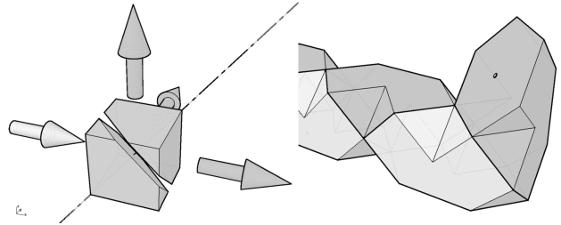
Fig. 1. Hexagonally bisected cube (Molecube) geometry, chained as C-motein. The Milli-Motein chain has this geometry, to allow it to form digitized approximations of arbitrary geometric shapes.
