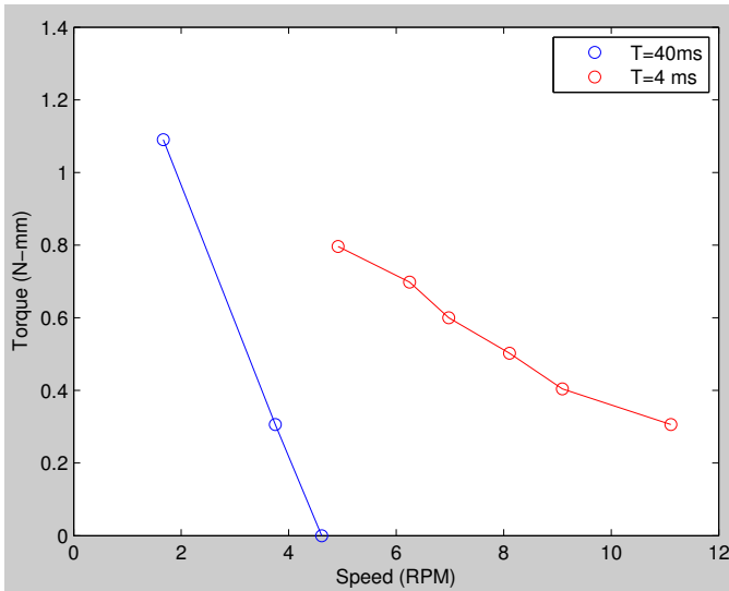
Fig. 8. Electropermanent stepper torque vs. speed curves, measured by hanging weights on a string from the rotor, and measuring the time for one revolution with a stopwatch. T is the time between switching pulses.
