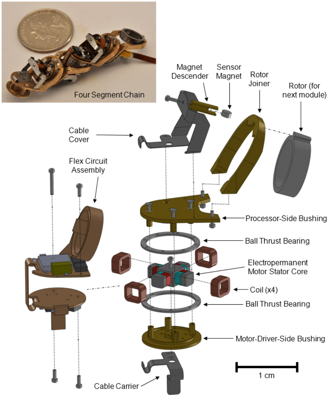
Fig. 5. This assembly is repeated for each joint. One segment of the continuous flex circuit is shown in its folded configuration. The stator on this module mates with the rotor on the adjacent module. See Figure 6 for an assembled view.
