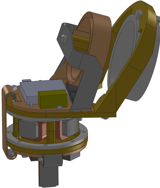
Fig. 6. This assembly is repeated for each joint. The stator on this module mates with the rotor on the adjacent module. See Figure 5 for an exploded view.
