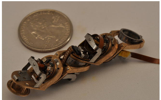
Fig. 2. Four segment Milli-Motein chain with a one centimeter module pitch. The chain folds itself into shapes using our new Electropermanent wobble motors.
