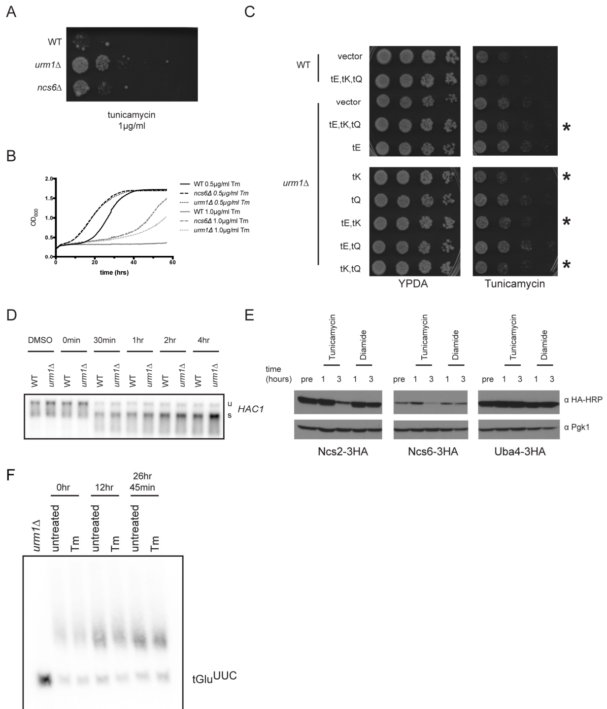
Figure 6. URM1 pathway mutants are resistant to tunicamycin in a tRNA dependent and HAC1 independent manner. (A) Five-fold serial dilutions of wild type, urm1Δ or ncs6Δ cells
