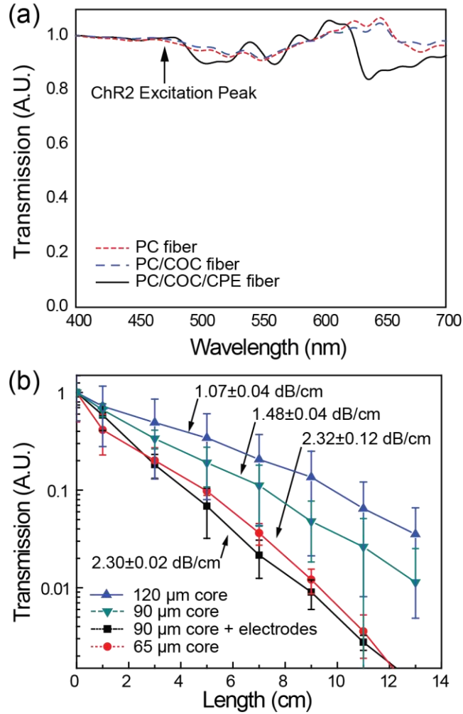
Figure 2: Optical characteristics of the fiber probe.
