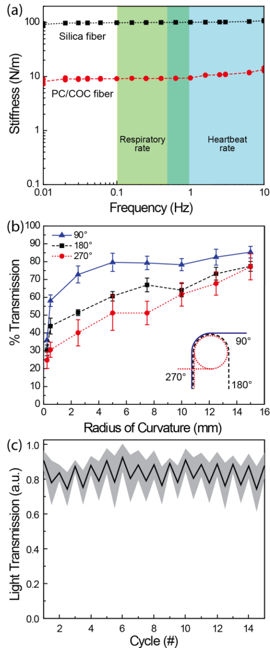
Figure 3: Mechanical characteristics of the fiber probe.
