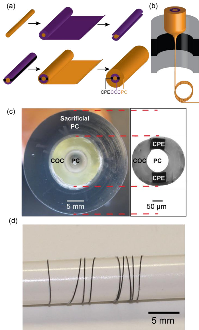
Figure 1: Fabrication process of all-polymer neural fiber probes.
