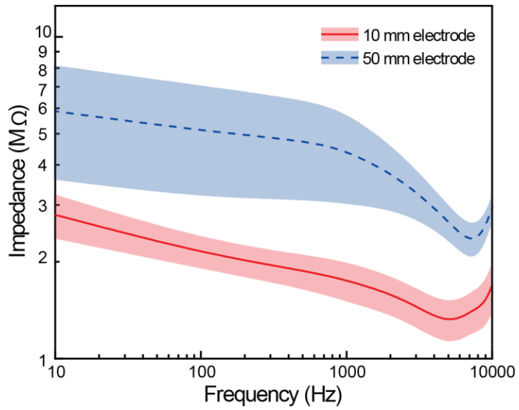
Figure 4: Embedded CPE electrode impedance.
