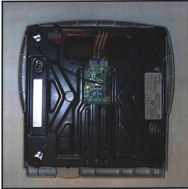
Figure 22: Transceiver Board in Scale
