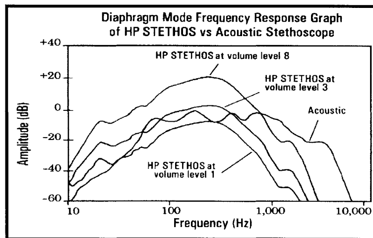
Figure 15: Stethos Frequency Response Chart
