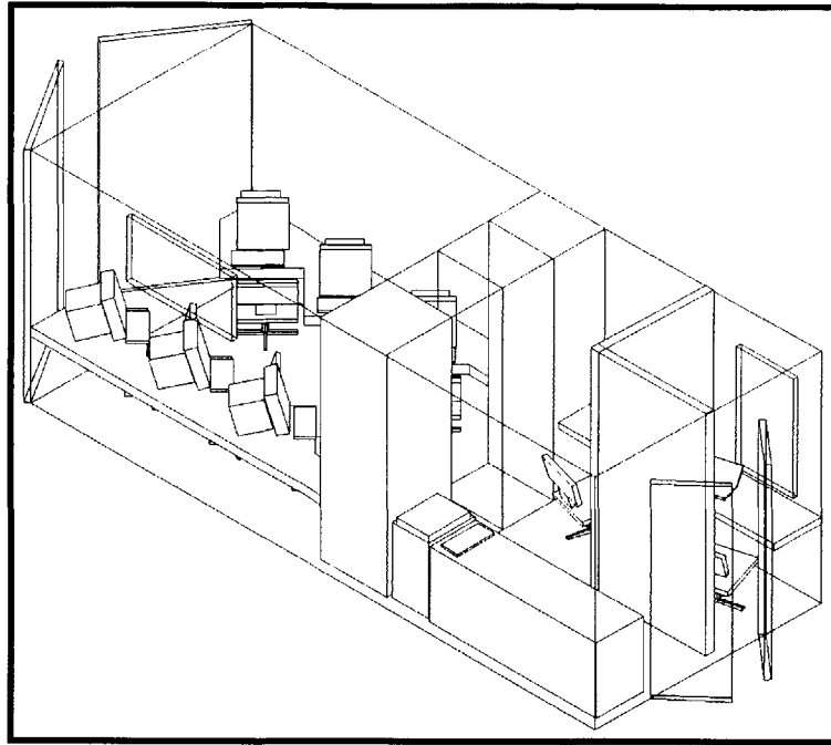
Figure 4: LINCOS Container Layout
