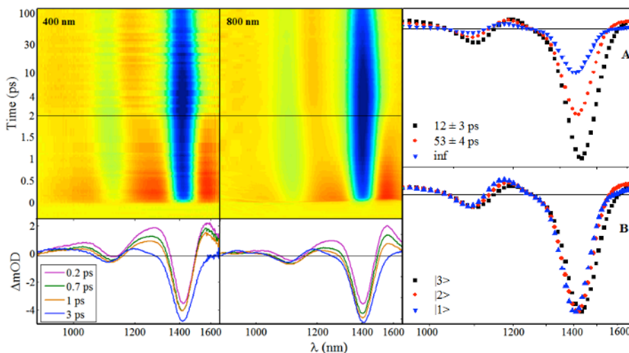
Fig. 1. Transient difference spectra presented above as \Delta OD maps, below as temporal cuts at the designated pump–probe delays, after excitation at 800 and 400 nm. SADS along with associated lifetimes after excitation at 800 nm (A) and normalized to the number of excitons (B) are presented in the right column
