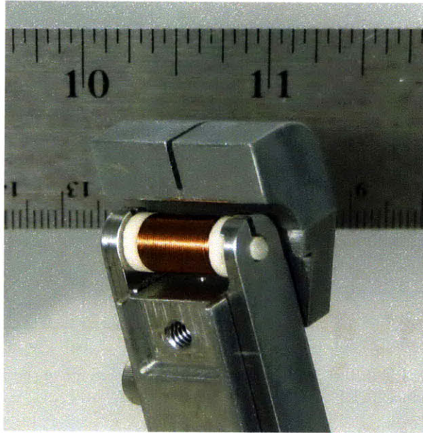
Figure 3-10: A pickup coil is mounted in a limiter with some shielding removed to show the assembly.
