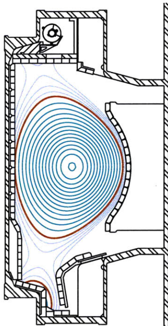
Figure 5-21: Equilibrium magnetic field reconstruction during a resonance in 1070626003. The red curve separates the confined field lines from the field lines the intersect vessel. This equilibrium is limited by the inner wall.
