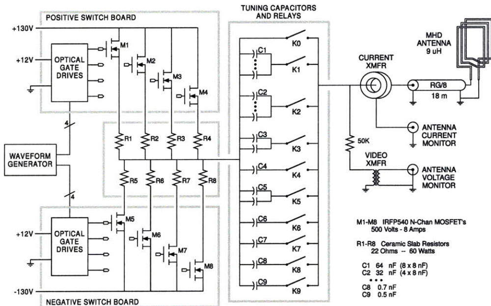
Figure 3-2: Each active MHD amplifier is composed of 8 N-channel MOSFETs. They can source \pm 130\text{V} and safely drive 23 A into a short. The effective output impedance is 5.5\Omega . A capacitive variable tuning network at the output of each amplifier matches the amplifier to the antenna impedance.
