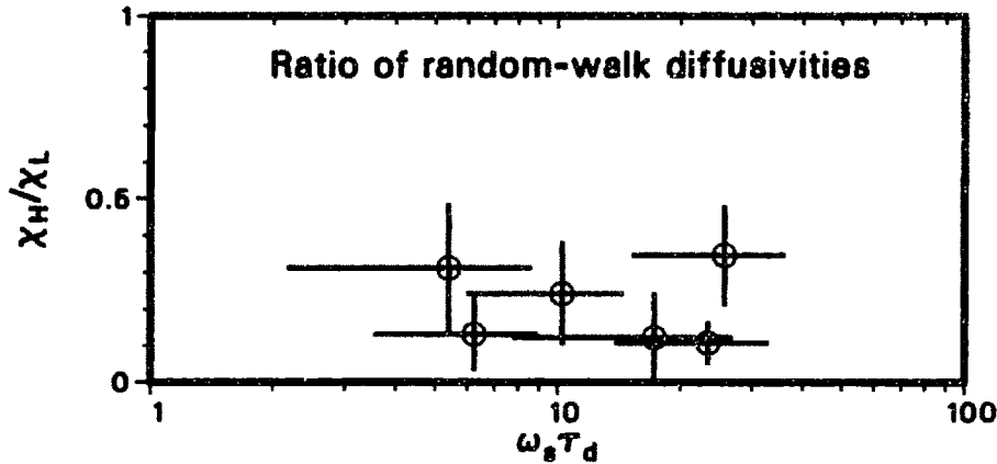
Fig. 6.11 Ratio of experimental random-walk diffusivities in H and L mode, as a function of the shearing rate multiplied by the intrinsic turbulence decorrelation time. The diffusivity is calculated as the square of the radial correlation length divided by the intrinsic decorrelation time: both quantities are determined from PCI measurements. The experimental values refer to the region 0.95 < \rho_n < 1.0 , where \rho_n is the normalized poloidal flux.
