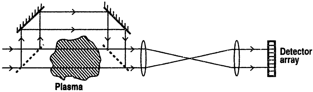
Fig. 2.13 Near-field Mach-Zehnder interferometer.
