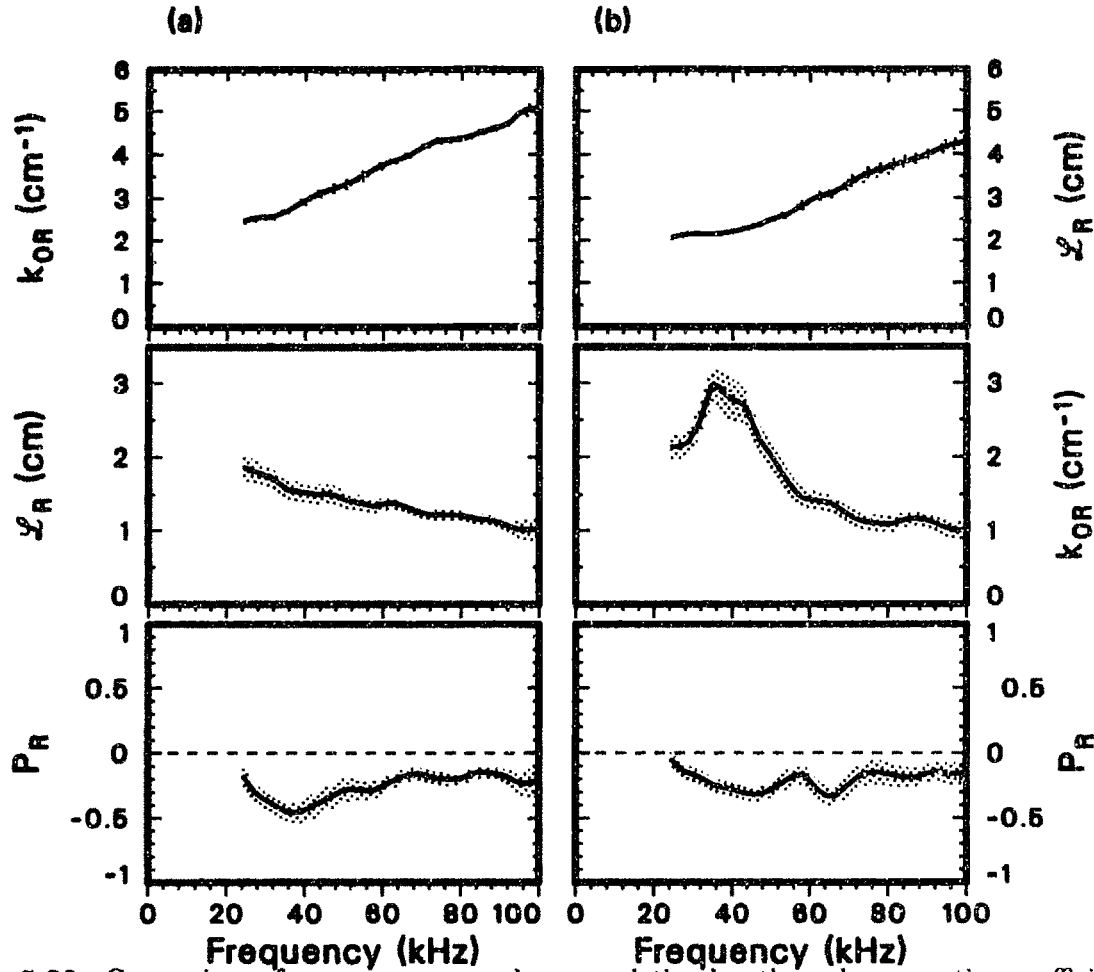
Fig. 5.20 Comparison of average wave number, correlation length, and propagation coefficient as functions of frequency for two different L-mode plasmas [(a) B_T=1.3 T, I_p=1.0 MA, \bar{n}_e=4\times 10^{13} cm ^{-3} , P_{\text{beam}}=0.6 MW, lower single-null); (b) B_T=2.16 T, I_p=1.35 MA, \bar{n}_e=4.5\times 10^{13} cm ^{-3} , P_{\text{beam}}=3.6 MW, double-null]. The measurements are made in the region between the LCFS and 3 cm inside. The shaded areas indicate confidence intervals. Smoothing was performed over a 10 kHz interval. The region below 24 kHz is not shown as it contained coherent MHD activity.
