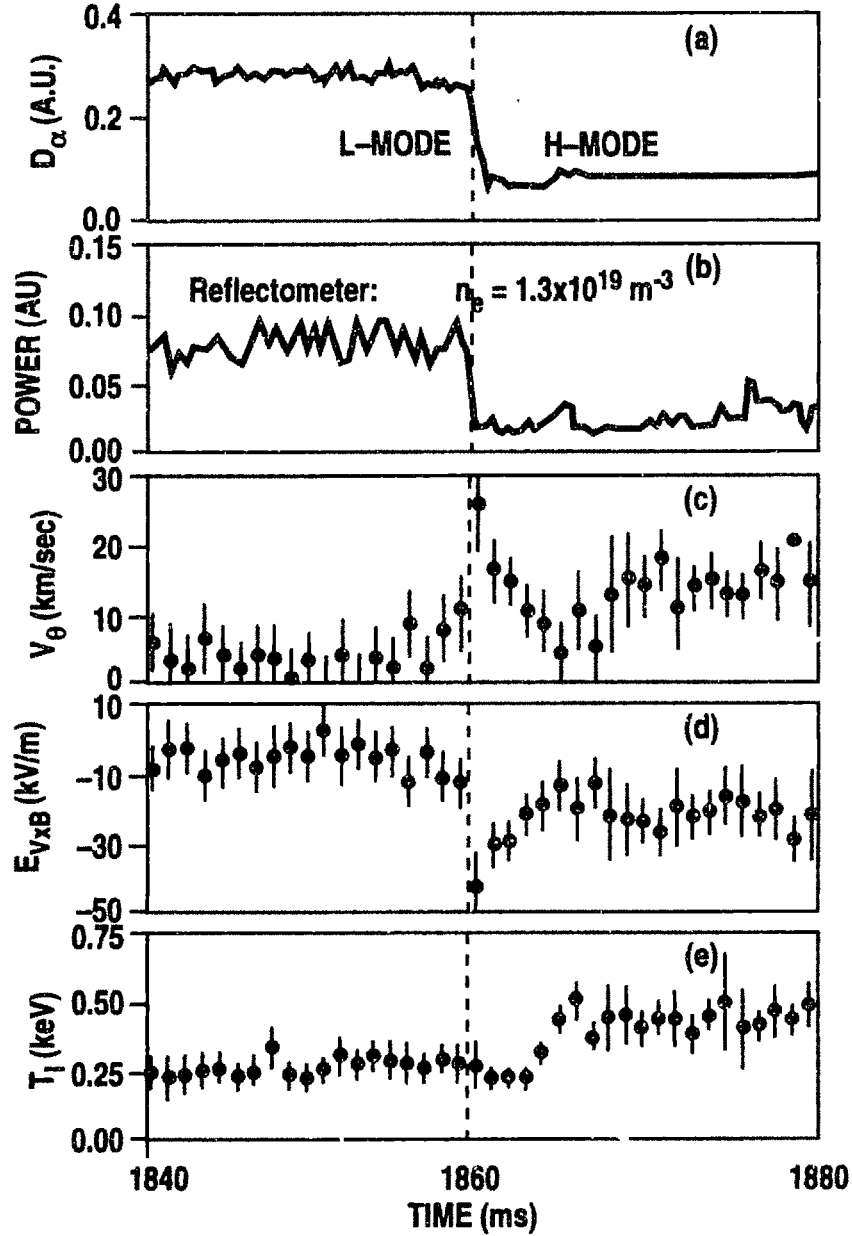
Fig. 1.2 Typical time evolution of fluctuation and rotation signals at an L-H transition: (a) the D_\alpha emission, which is a measure of edge transport, drops at the transition; (b) integrated fluctuation power in the 75–400 kHz band, measured by a reflectometer a few cm inside the last closed flux surface; (c), (d) and (e) show the poloidal rotation velocity, the radial electric field, and the ion temperature measured by charge-exchange recombination spectroscopy \sim 1 cm inside the last closed flux surface [reproduced with permission from E.J. Doyle, et al., Phys. Fluids B 3, 2300 (1991).]
