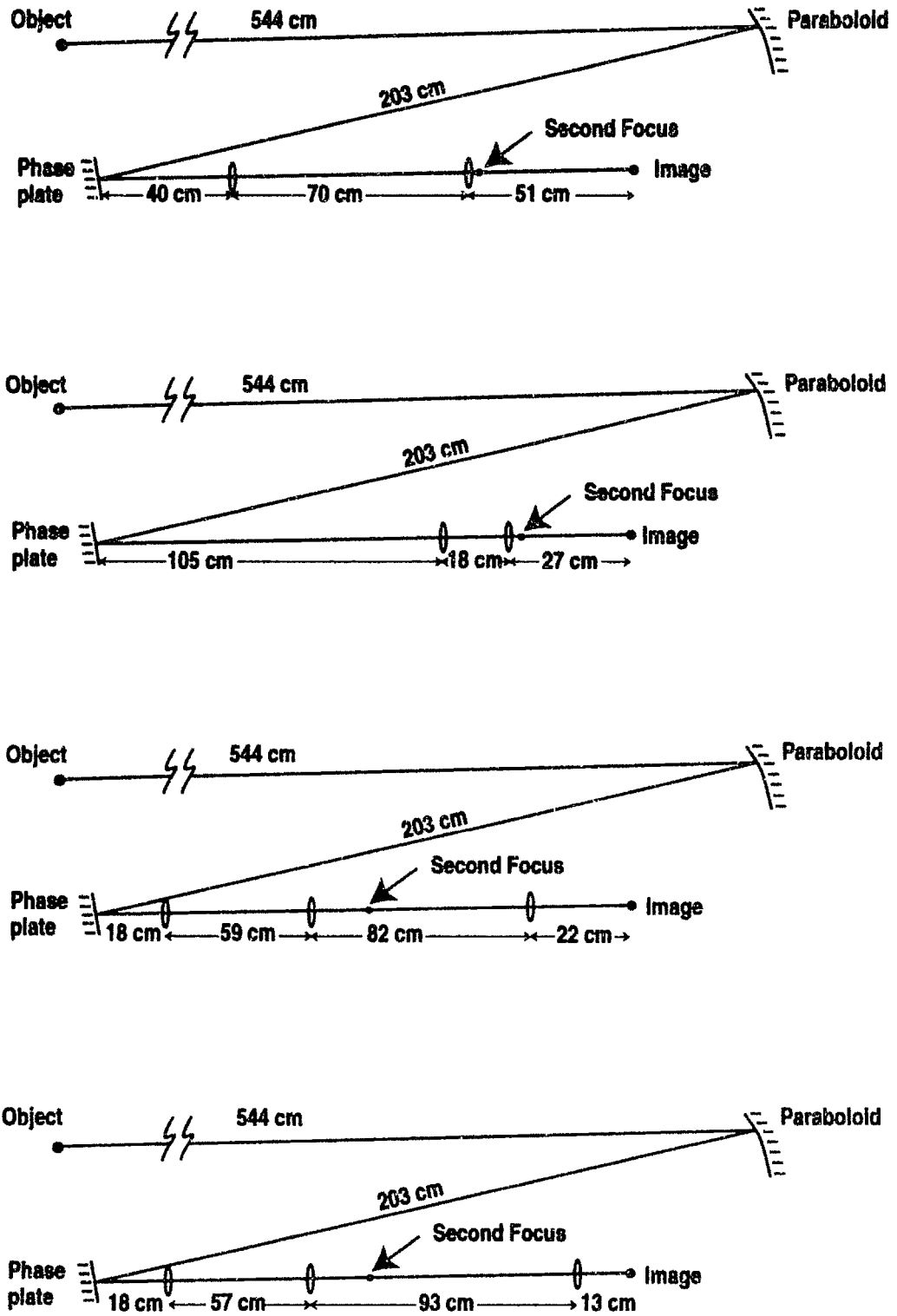
Fig. 3.10 Imaging geometries.
