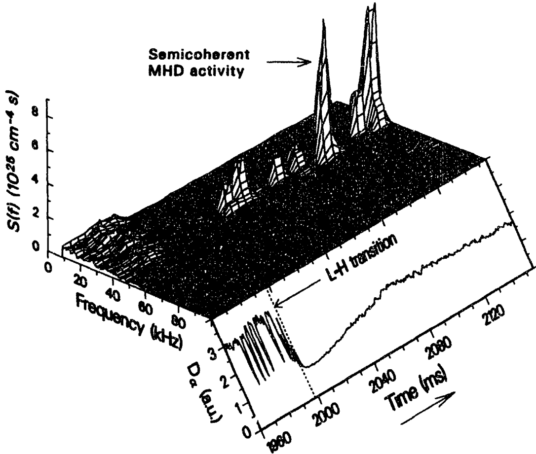
Fig. 5.60 Three-dimensional plot of the time history of the PCI autopower spectrum on a chord located 0.4 cm inside the LCFS, and time trace of the D_{\alpha} line emission from the divertor. A smoothing interval of 2 kHz was used to estimate the autospectrum, with a statistical uncertainty of 22%. The absolute calibration error on the power is 45%. The plasma parameters are B_T=2.16 T, I_p=1.65 MA, \bar{n}_e=4.5 \times 10^{13} cm ^{-3} , and input power = 14 MW.
