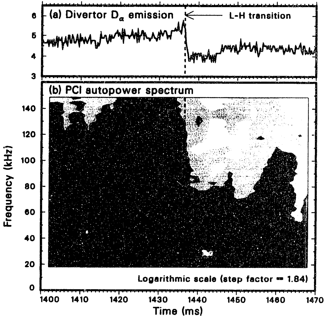
Fig. 5.36 (a) Time trace of the D_\alpha line emission from the divertor and (b) contour plot in logarithmic scale of the time evolution of the PCI autopower spectrum 0.3 cm inside the LCFS, across the L-H transition (the level is proportional to the logarithm of the intensity). A smoothing interval of 20 kHz was used to estimate the autospectrum, with a statistical uncertainty of 11%. The plasma parameters are B_T=2.0 T, I_p=1.64 MA, \bar{n}_e=3.8\times 10^{13} cm ^{-3} , and input power = 13 MW.
