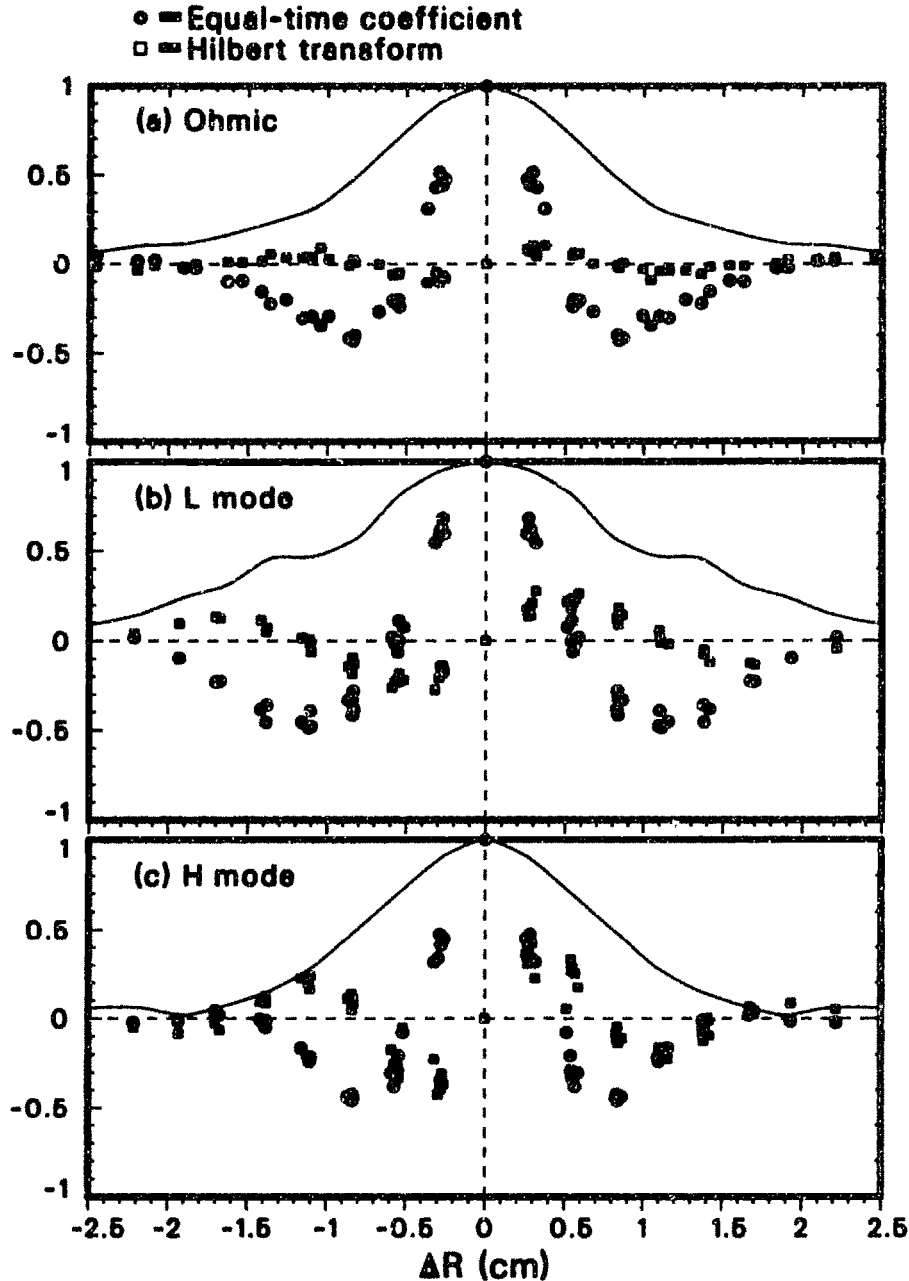
Fig. 5.8 Equal-time coefficient and its Hilbert transform for three cases: (a) Ohmic ( B_T=2.1 T, I_p=1.9 MA, \bar{n}_e=3 \times 10^{13} cm ^{-3} , input power = 3.5 MW), (b) L mode and (c) H mode (both B_T=2.1 T, I_p=1.25 MA, \bar{n}_e=3.5 \times 10^{13} cm ^{-3} , input power = 6.2 MW). The solid curves represent the envelopes of the equal-time coefficient. The plots refer to the region between the LCFS and 3 cm inside. The 95% confidence level is 0.02. Fits give correlation lengths, respectively, of 1.2 cm, 1.5 cm, and 1.2 cm; and average wave numbers of 3.4 cm ^{-1} , 2.8 cm ^{-1} , and 3.9 cm ^{-1} .
