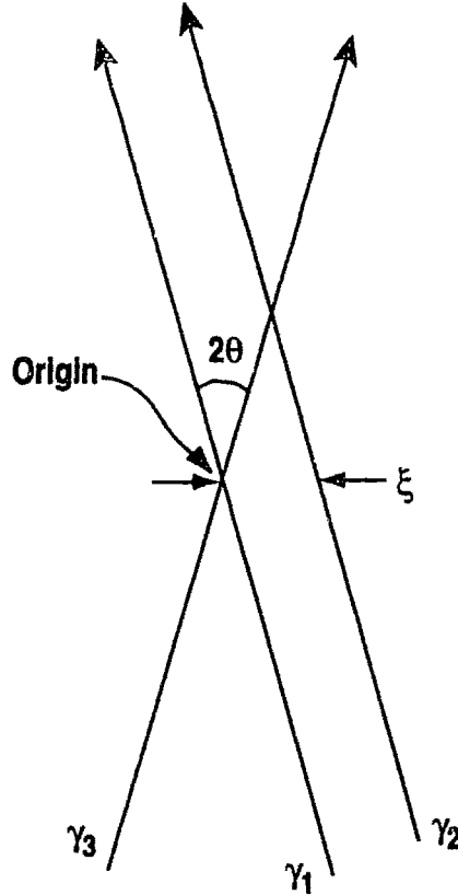
Fig. 7.9 Three-chord correlation geometry.
