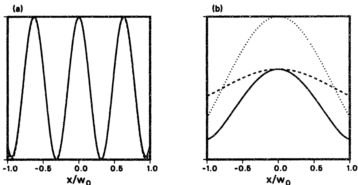
Fig. 2.23 Comparison of a sample sinusoidal \bar{n}_e function (dotted line), of the corresponding phase-contrast signal calculated by means of the approximate response function (dashed line), and of the exact phase-contrast signal calculated with a convolution integral (solid line), for (a) kw_0/2 = 5 , (b) kw_0/2 = 1 . Here, Q=1.5 and \alpha=1 .
