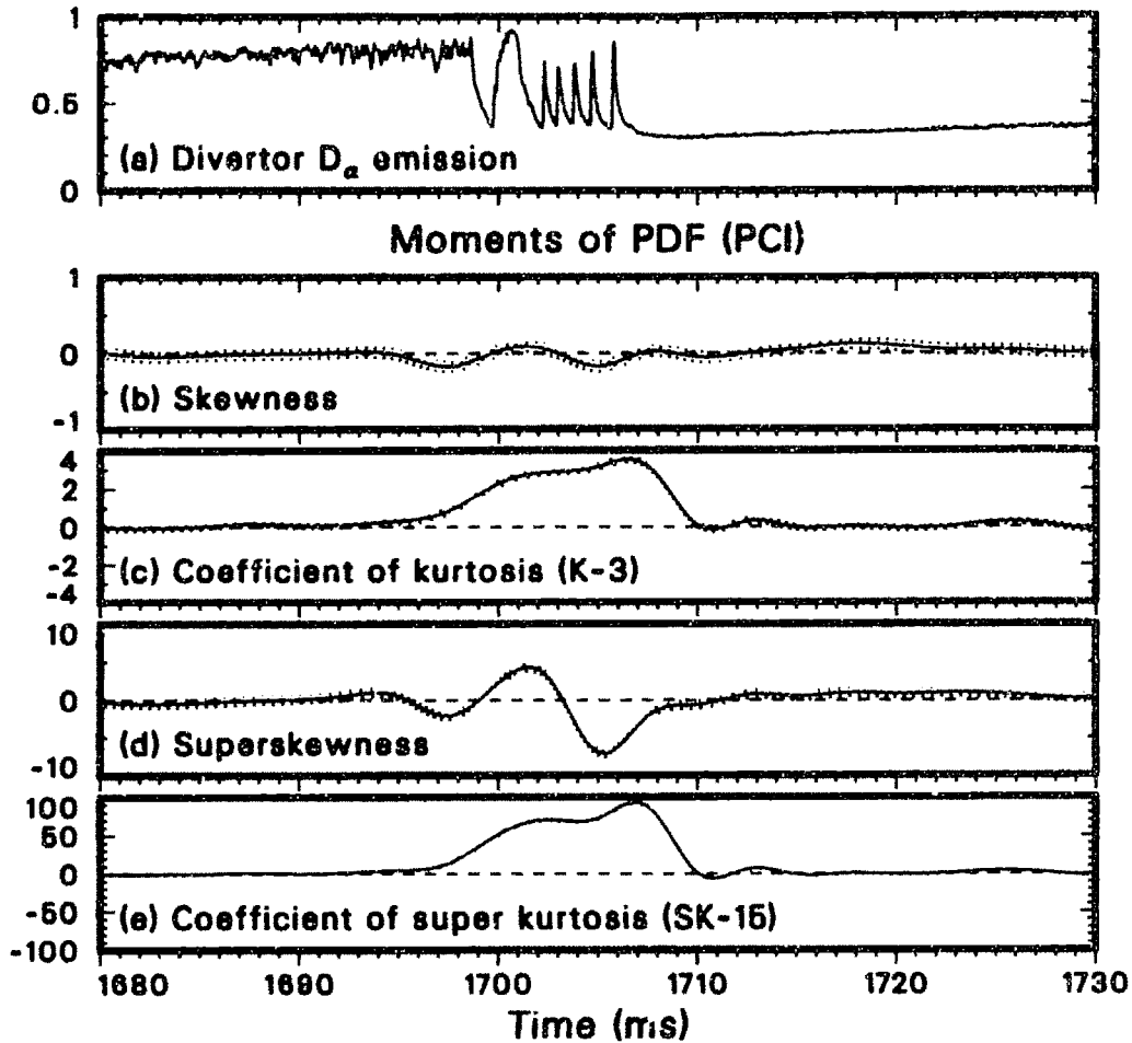
Fig. 5.42 (a) D_\alpha line emission from the divertor, and (b–e) third, fourth, fifth, and sixth moment of the PCI probability distribution function (PDF), minus the Gaussian value (respectively 0, 3, 0, 15). The dithering L–H transition is indicated by the drop in the D_\alpha signal. The PDF is estimated over half-overlapped 5-ms intervals (2500 samples), with a bin size equal to 0.1 standard deviations; the moments are calculated over a range of six standard deviations. The PCI major radius at the midplane is 3.4 cm inside the LCFS. The shaded areas indicate confidence intervals. The plasma parameters are B_T=2.1 T, I_p=1.25 MA, \bar{n}_e=3.5 \times 10^{13} cm ^{-3} , input power = 6.2 MW.
