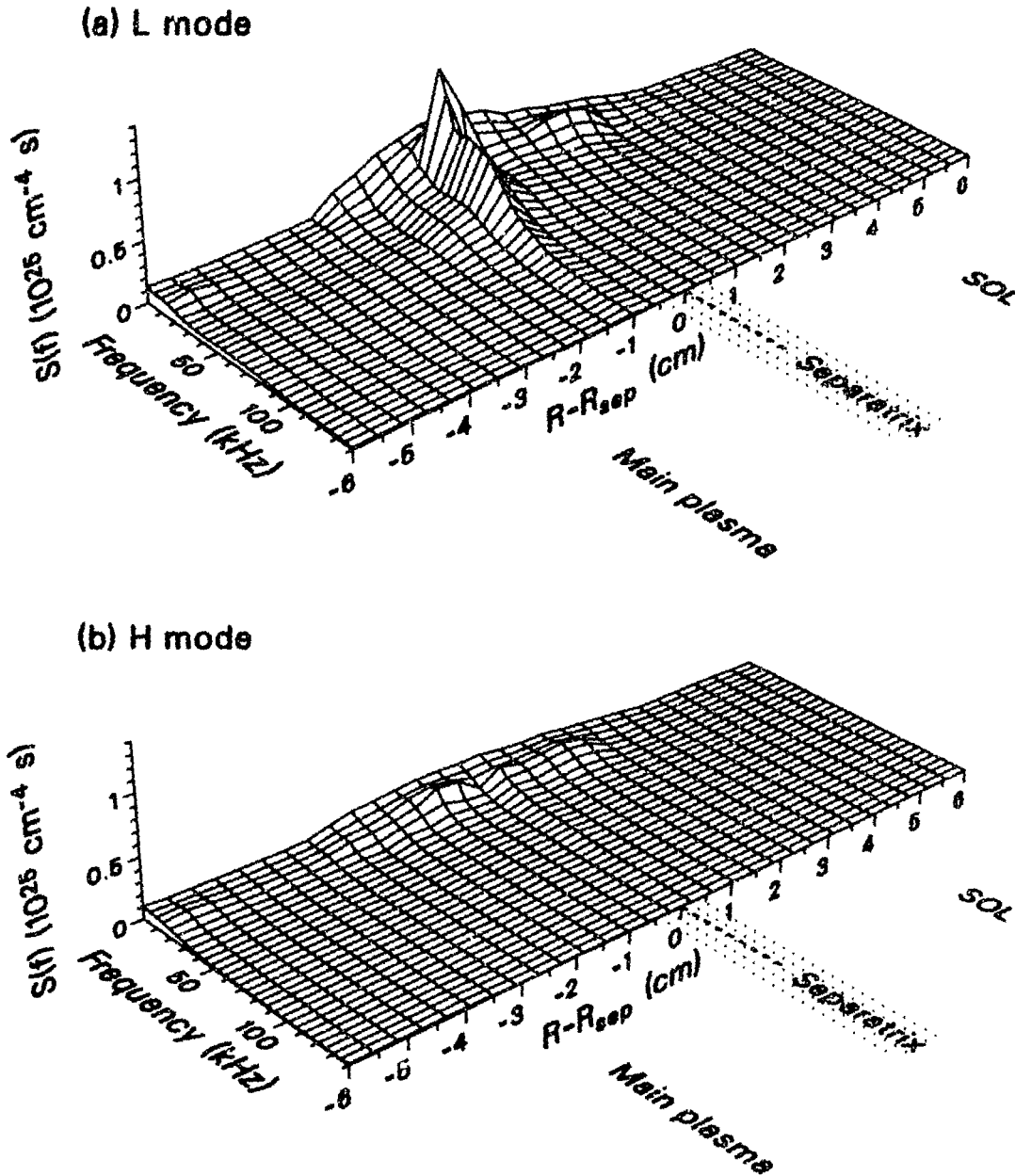
Fig. 5.27 Radial profiles of frequency autospectra of calibrated line integrals of \tilde{n} , in (a) L mode and (b) H mode. Data collected from a set of similar shots (same as in Fig. 5.26) with varying separatrix position ( B_T=2.1 T, I_p=1.35 MA, \bar{n}_e=4\times 10^{13} cm ^{-3} , P_{\text{beam}}=1.1\text{--}2.3 MW, lower single-null). Smoothing was performed over a 10 kHz interval. Relative error bars (not shown) are \sim 10\% ; the uncertainty on the absolute calibration is 40%.
