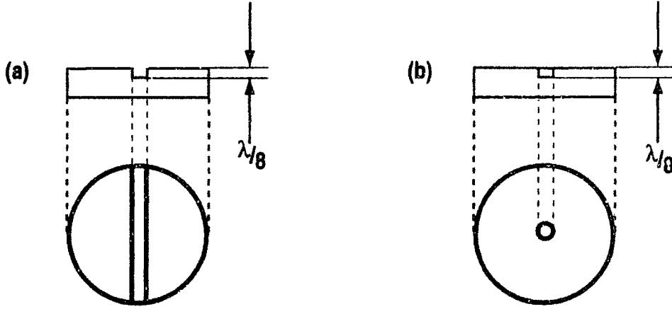
Fig. 2.17 Reflective phase plate, (a) one-dimensional and (b) two-dimensional.
