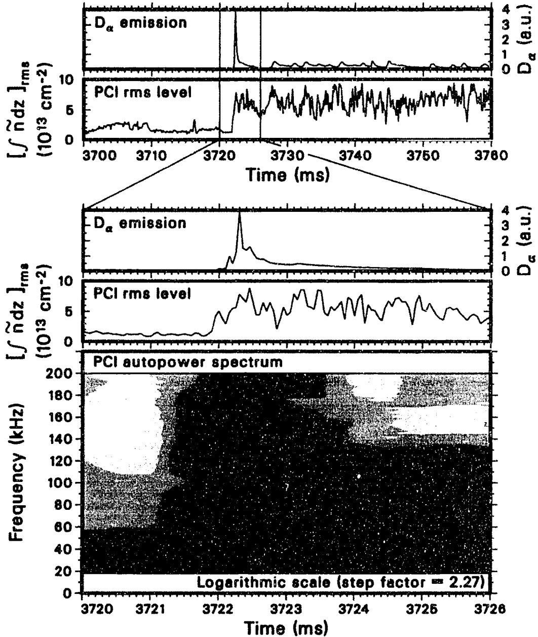
Fig. 5.58 Time traces of the D α line emission from the divertor and of the PCI rms level (top); blowup of the same traces for an X event, and contour plot in logarithmic scale of the time evolution of the PCI autopower spectrum (bottom; the level is proportional to the logarithm of the intensity). The PCI chord intersects the midplane 1.2 cm inside the LCFS. The statistical error on the rms level is 10%; the absolute amplitude calibration error is 30%. A smoothing interval of 20 kHz was used to estimate the autospectrum, with a statistical uncertainty of 22%. The plasma parameters are B_T=2.16 T, I_p=2.0 MA, \bar{n}_e=9\times 10^{13} cm -3 , and input power = 5.5 MW.
