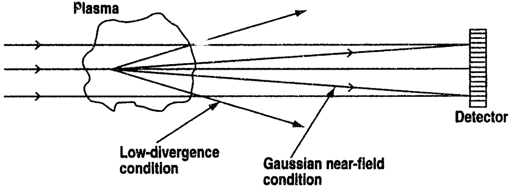
Fig. 2.10 Illustration of low-divergence condition (scattered waves stay within the Gaussian cross section in the plasma) and more stringent Gaussian near-field condition (scattered waves stay within the Gaussian cross section at the detector).
