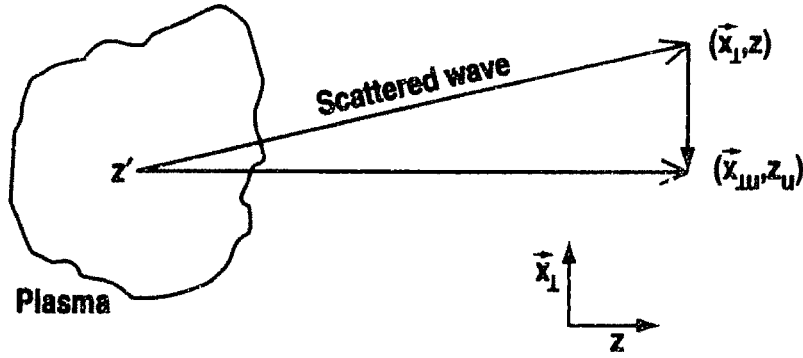
Fig. 2.6 Unperturbed coordinates.
