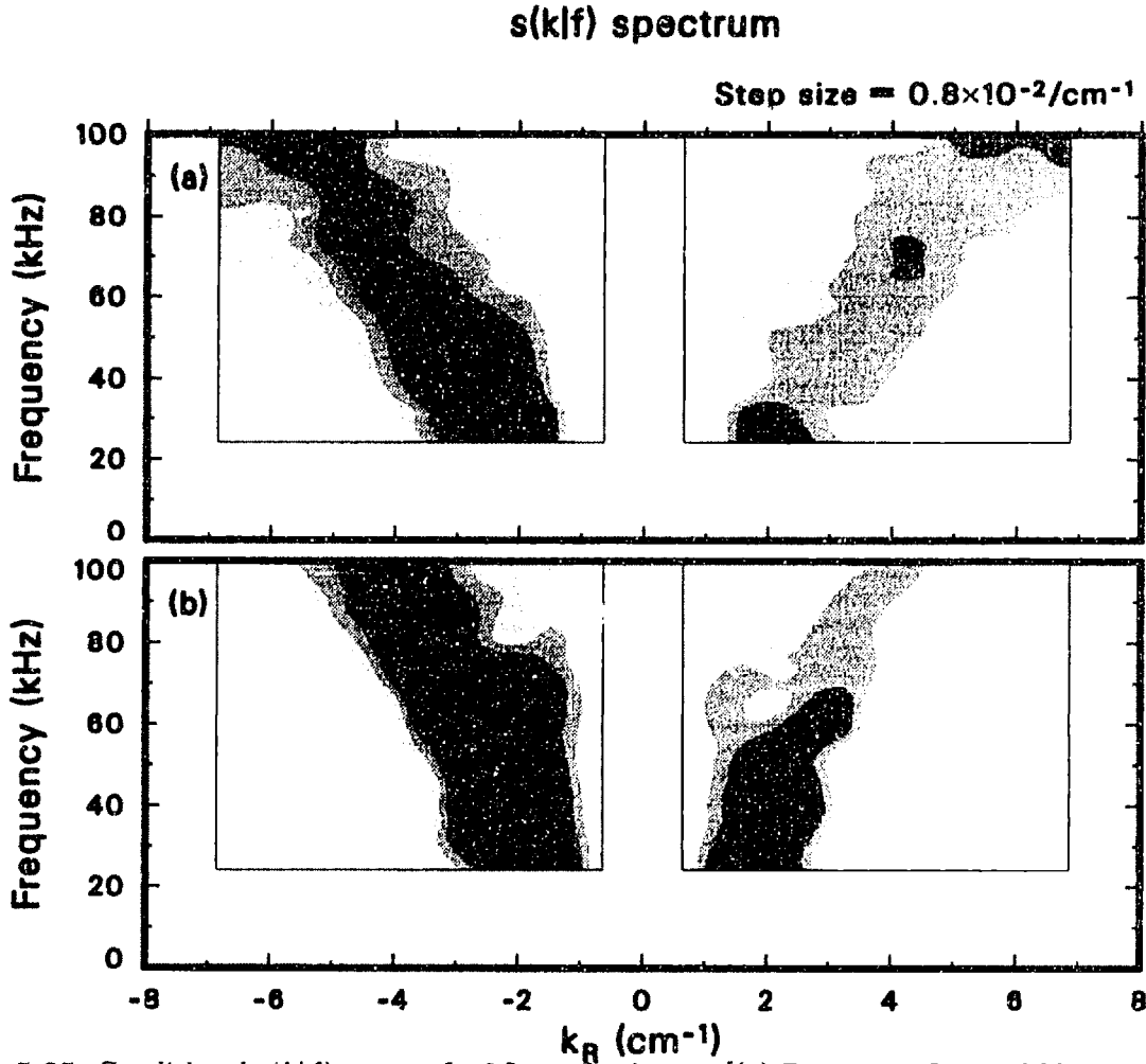
Fig. 5.25 Conditional s(k|f) spectra for 2 L-mode plasmas [(a) B_T=1.3 T, I_p=1.0 MA, \bar{n}_e=4 \times 10^{13} \text{cm}^{-3} , P_{\text{beam}}=0.6 MW, lower single-null); (b) B_T=2.16 T, I_p=1.35 MA, \bar{n}_e=4.5 \times 10^{13} \text{cm}^{-3} , P_{\text{beam}}=3.6 MW, double-null], corresponding to the cases of Fig. 5.20. The measurements are made in the region between the LCFS and 3 cm inside. The integral of S over wave numbers at each frequency is equal to one. Smoothing was performed over a 10 kHz interval. The region below 24 kHz is not shown as it contained coherent MHD activity.
