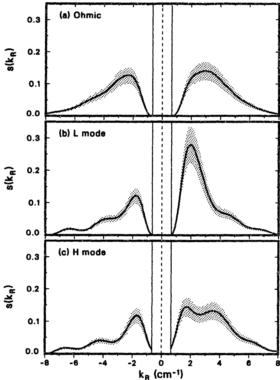
Fig. 5.17 Normalized radial wave-number spectra in the region between the LCFS and 3.5 cm inside, for three cases: (a) Ohmic ( B_T=2.1 T, I_p=1.9 MA, \bar{n}_e=3 \times 10^{13} \text{cm}^{-3} , input power = 3.5 MW), (b) L mode and (c) H mode (both B_T=2.1 T, I_p=1.3 MA, \bar{n}_e=3 \times 10^{13} \text{cm}^{-3} , P_{\text{beam}}=15 MW). The shaded areas represent confidence intervals. The spectra are normalized to an integral of 1. The blank region near k = 0 is below the instrumental cutoff. Case (a) corresponds to Fig. 5.8(a).
