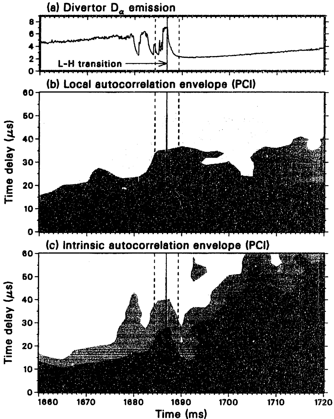
Fig. 5.41 (a) D_\alpha line emission from the divertor, (b) contour plot of envelope of local (3.4 cm inside the LCFS) time-delayed autocorrelation function, (c) contour plot of envelope of intrinsic autocorrelation function in the region between 3.5 and 5 cm inside the LCFS. The step size in the contour plots is 0.11; the 95% confidence level is 0.05; the level is proportional to the intensity. The resolution of the correlation estimate is \pm 2.5 ms, as indicated by the dashed lines around the L-H transition. The plasma parameters are B_T=2.1 T, I_p=1.3 MA, \bar{n}_e=3 \times 10^{13} cm ^{-3} , input power = 15 MW.
