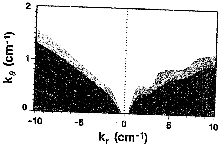
Fig. 4.18 Responsivity of the PCI system to individual (k_r, k_\theta) modes.
