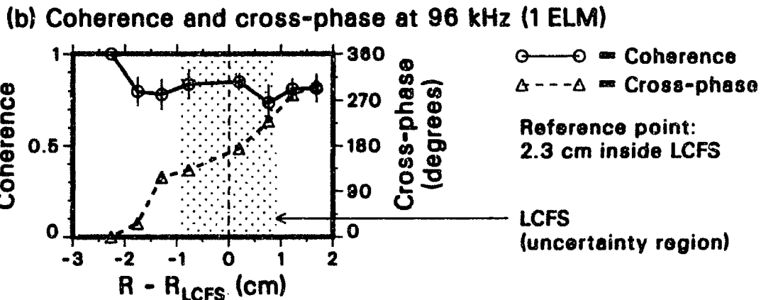
Fig. 5.56 (a) Three-dimensional plot of the evolution in time of the PCI autopower spectrum 1.7 cm inside the LCFS (estimated over a 20-kHz smoothing interval, with a statistical uncertainty of 16%), and time trace of the D_\alpha line emission from the divertor; (b) coherence and cross-phase with respect to a chord located 2.3 cm inside the LCFS, plotted as a function of the distance from the LCFS (with maximum statistical errors of, respectively, 11% and 8^\circ ). The positive slope in the phase function indicates outward propagation; a cosine fit to the complex coherency function gives a wavelength of 4.5 cm. The discharge is the same as for Figs. 5.54 and 5.55. The plasma parameters are B_T=2.1 T, I_p=1.0 MA, \bar{n}_e=5.5 \times 10^{13} cm ^{-3} , and input power = 6.9 MW.
