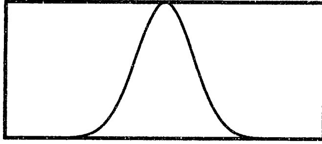
Fig. 2.3 Gaussian function.
