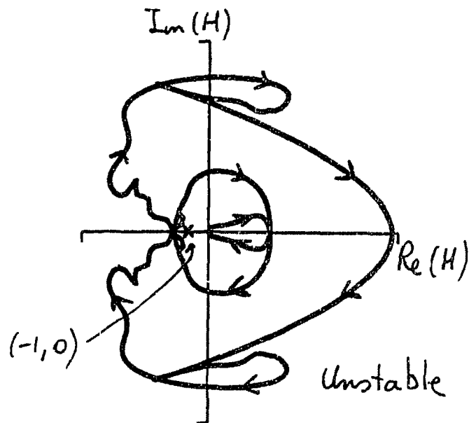
Fig. 3.19 (a) Nyquist contour; (b) mapping for H(s) = PCS(s) , for a stable case (top) and an unstable case (bottom).
