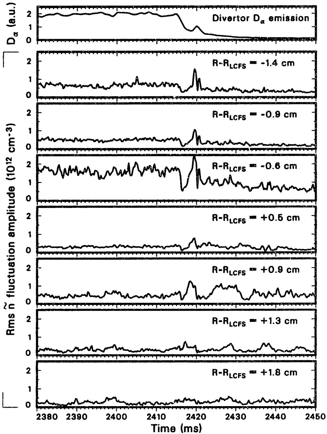
Fig. 5.35 Time traces of the D_\alpha line emission from the divertor and of the rms density fluctuation amplitude at seven radial locations: the top three curves correspond to locations inside the LCFS, and the bottom four curves refer to the SOL. The L-H transition is identified by the drop in the D_\alpha signal. The systematic error on the rms fluctuation level is estimated at 40% and the random error from channel to channel is 18%. The plasma parameters are B_T=2.1 \text{ T} , I_p=1.37 \text{ MA} , \bar{n}_e=4 \times 10^{13} \text{ cm}^{-3} , input power = 1.9 MW.
