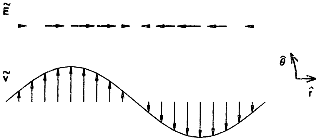
Fig. 6.1 Two-dimensional vector diagram of fluctuating electric field and corresponding \mathbf{E} \times \mathbf{B} velocity for a single radial mode.
