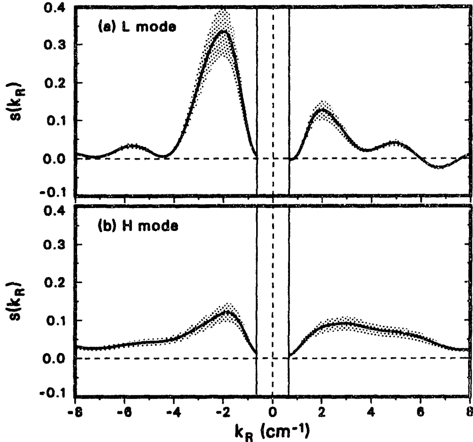
Fig. 5.18 Normalized radial wave-number spectra in the region between the LCFS and 3 cm inside, in (a) L mode (input power = 2.7 MW) and (b) H mode (3.0 MW). Plasma parameters are B_T=2.1 T, I_p=1.35 MA, \bar{n}_e=4 \times 10^{13} \text{cm}^{-3} . The shaded areas represent confidence intervals. The spectra are normalized to an integral of 1. The blank region near k = 0 is below the instrumental cutoff. Case (a) corresponds to Fig. 5.12(a), case (b) to Fig. 5.13(a).
