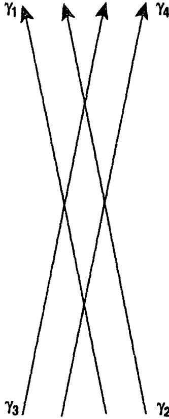
Fig. 7.10 Four-chord correlation geometry.
