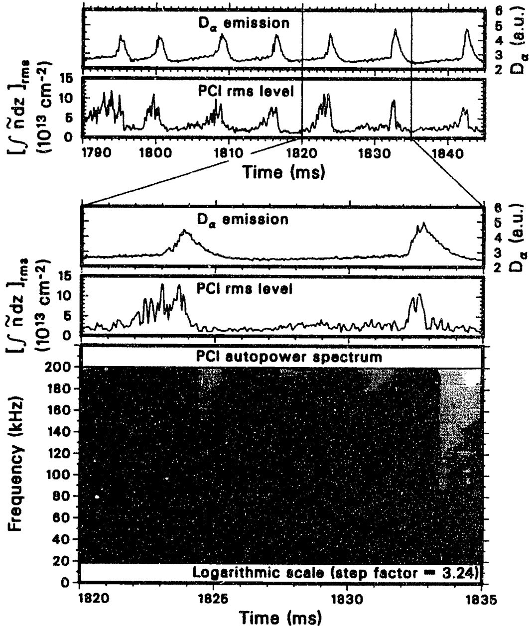
Fig. 5.52 Time traces of the D_\alpha line emission from the divertor and of the PCI rms level (top); blowup of the same traces for two type-I ELMs, and contour plot in logarithmic scale of the time evolution of the PCI autopower spectrum (bottom; the level is proportional to the logarithm of the intensity). Precursor activity is seen before the first ELM in the blowup, but not before the second one. The PCI chord intersects the midplane 0.5 cm inside the LCFS. The statistical error on the rms level is 10%; the absolute amplitude calibration error is 40%. A smoothing interval of 20 kHz was used to estimate the autospectrum, with a statistical uncertainty of 22%. The plasma parameters are B_T=2.1 T, I_p=1.25 MA, \bar{n}_e=3.5 \times 10^{13} \text{ cm}^{-3} , input power = 6.2 MW.
