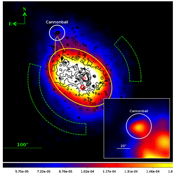
Figure 1. NuSTAR mosaic image of the Cannonball, Plume, and Sgr A* region in 3–79 keV band. The Cannonball is indicated by the white circle with radius of 20'' . Background regions are indicated by the green dashed regions. Chandra 3–8 keV contours are overlaid in black, and approximate positions of the Plume and Sgr A East are in yellow. The image is shown with a linear color scale and the scale range chosen to highlight the Cannonball emission. Inset: NuSTAR mosaic image of the Cannonball in 10–30 keV band.
