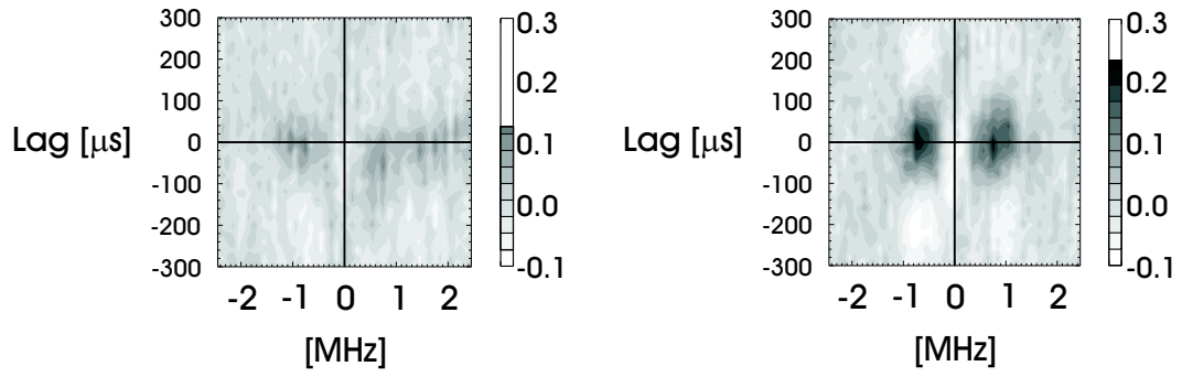
FIG. 18: Cross correlation between Mirnov rms signal and density fluctuation band autopower (volume 2) vs band frequency and time lag (units of 20 \mu\text{s} ). Left: Shot 47941 (SG), right: Shot 47944 (SB).
