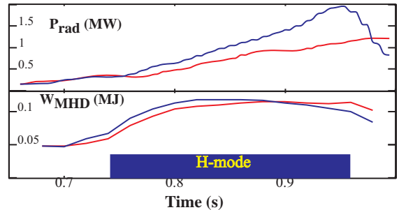
Figure 5: Comparison of D(H) blue and D( 3 He) H-mode following boronization shows little difference in stored energy.
