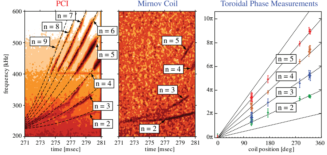
FIG. 2: (color online) (a) Spectrogram of RSAEs excited during a sawtooth cycle as measured by PCI, with mode numbers inferred from the best fit to Eq. 1 overlaid in dashed line. (b) Spectrogram for the same time period measured by a Mirnov coil. (c) Measured phases of the modes detected by the Mirnov coils as a function of toroidal angle, confirming the inference from the PCI analysis.
