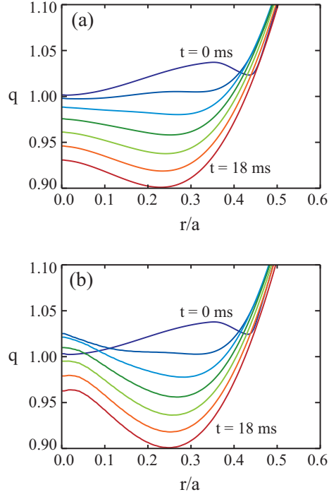
FIG. 8: (color online) Evolution of q profiles during a sawtooth cycle of 18ms at equal time intervals of 3ms. The initial conditions are provided by the Kadomtsev model results similar to those presented in Fig. 7. The two cases are (a) classical resistivity with flat Z_{eff} profile and (b) neoclassical resistivity with peaked Z_{eff} profile.
