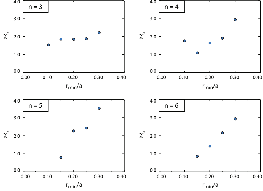
FIG. 5: (color online) \chi^2 as a function of r_{min}/a for the n=3,4,5,6 modes identified in Fig. 2 show a best-fit solution near r_{min}/a = 0.15 . No solutions at r_{min}/a = 0.10 were found for the n=5 and 6 cases.
