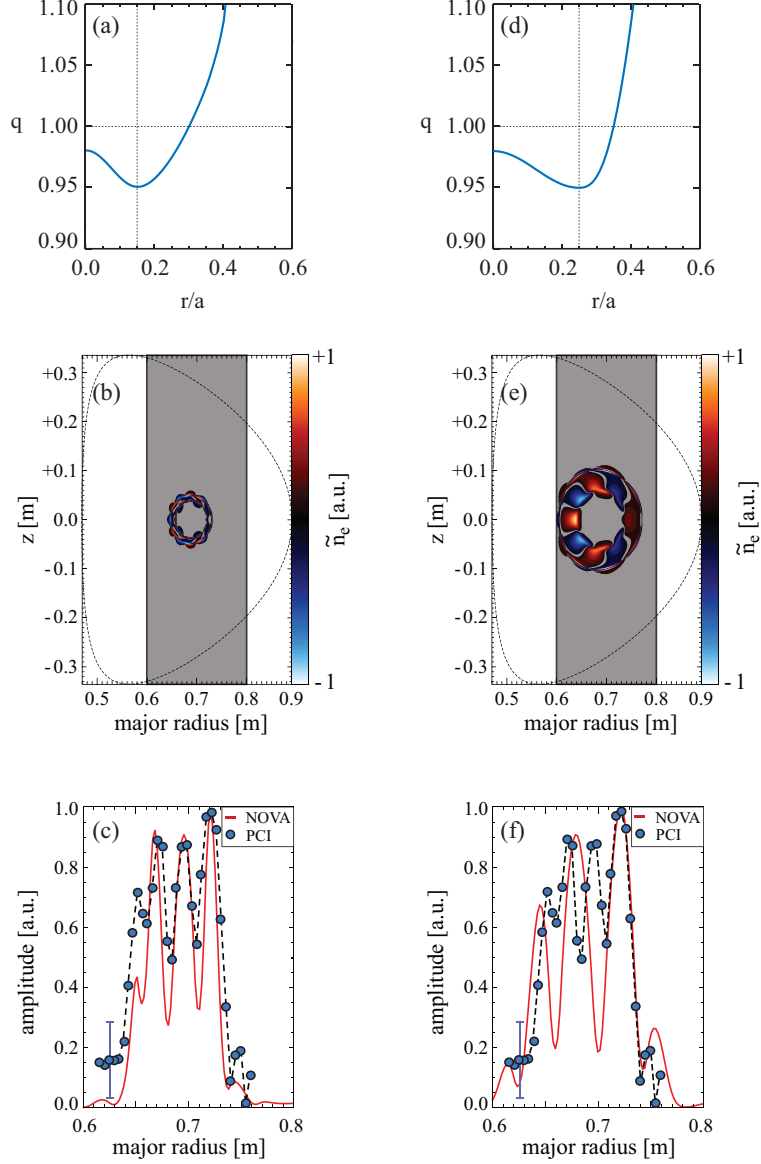
FIG. 3: (color online) The synthetic PCI analysis shows the greatest sensitivity to r_{min} , which manifests as the peak spacing and width in the synthetic signal. (a) The input q profile with q_{min} = 0.95 , q_0 = 0.98 , r_{min}/a = 0.15 . (b) The the two dimensional density perturbation calculated by NOVA for an n=4 RSAE using the above q profile and (c) the resulting comparison between the experimental and synthetic PCI signals. Panels (d)-(f) use an un-optimized value of r_{min}/a = 0.25 to illustrate the differences in synthetic diagnostic signal.
