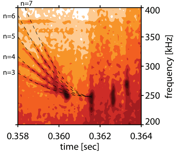
FIG. 6: (color online) PCI spectrogram of down-chirping RSAEs immediately following a sawtooth crash. Toroidal mode numbers of n=3-7 are identified by comparison with Eq. 1 which implies that q_{max} \approx 1.03 following the crash.
