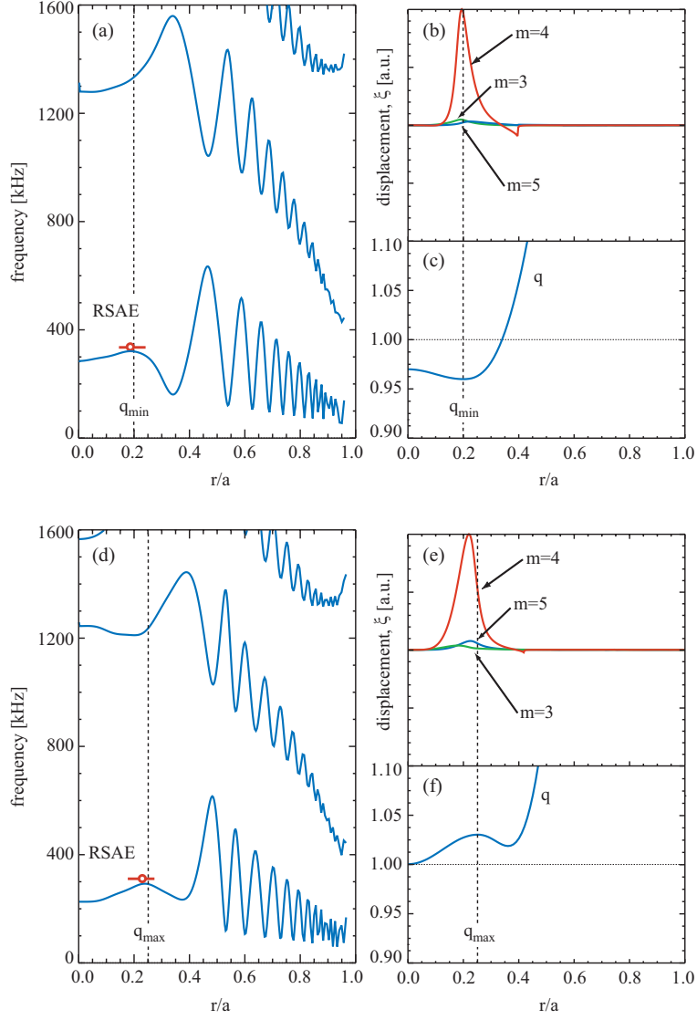
FIG. 4: (color online) (a) Alfvén continuum plot from NOVA for an n=4 up-chirping RSAE. (b) The radial displacement eigenmode associated with the q profile shown in (c). Plots (d)-(f) pertain to a down-chirping RSAE for a q profile with a local maximum at r/a = 0.25 .
