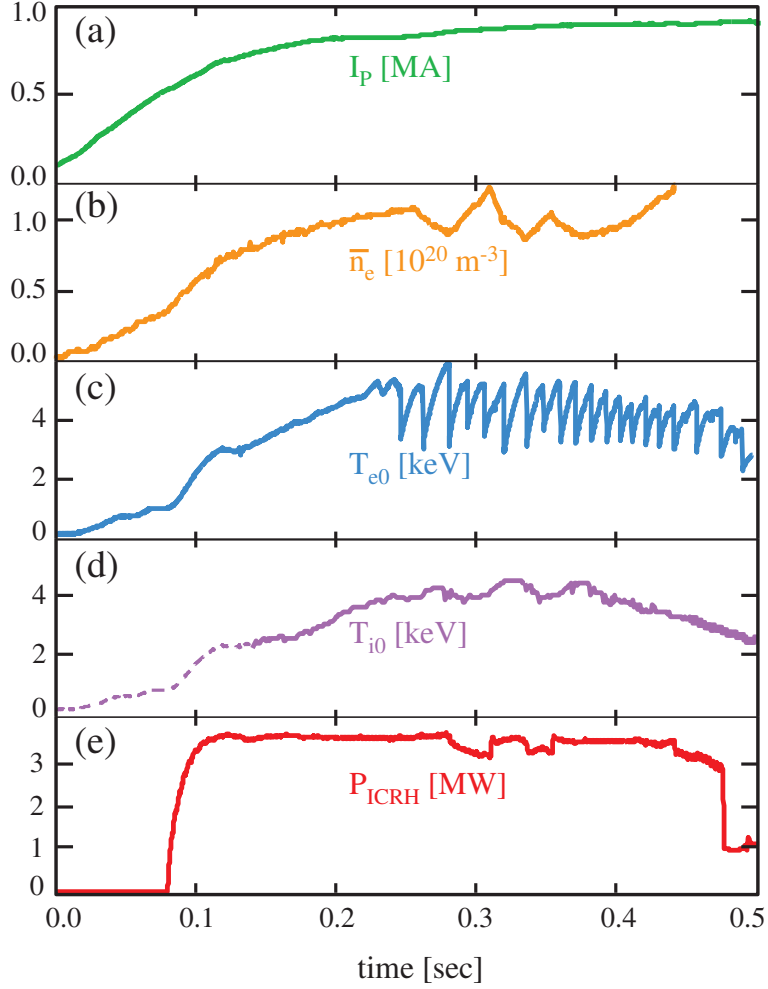
FIG. 1: (color online) Experimental traces showing (a) total plasma current (b) line-averaged electron density (c) central electron temperature from the ECE diagnostic (d) central deuterium ion temperature derived from the neutron flux and (e) the injected ICRH power. The breaks in slope of the density trace, starting around 0.25 seconds, indicate transitions between L-mode and ELM-free H-Mode. No ion temperature data is available before 0.15 seconds and is represented as 0.8 times T_{e0} for this time range (dashed trace).
