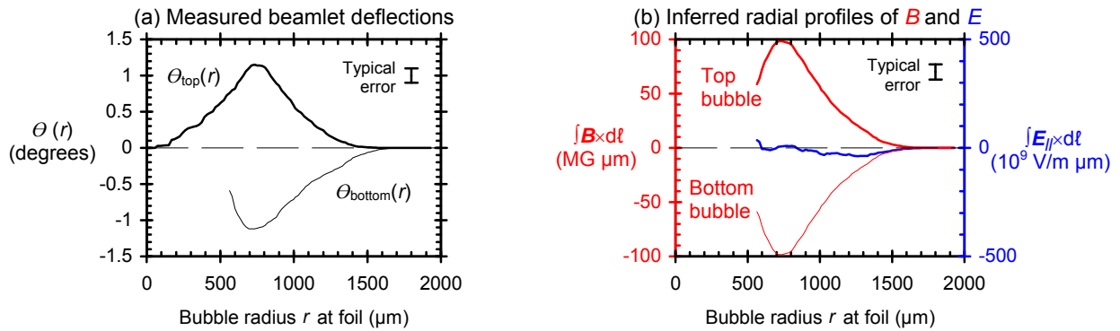
FIG. 2 (color). Measured beamlet deflection angles \theta as a function of radius r in the top and bottom bubbles of Fig. 1(b) (positive is away from the bubble center), and inferred radial profiles of |\mathbf{B} \times d\mathbf{l}| and |\mathbf{E}_{\parallel} \times d\mathbf{l}| in the two bubbles. In (b), the vector |\mathbf{B} \times d\mathbf{l}| is plotted as a positive number for a toroidal \mathbf{B} field in the clockwise direction of Fig. 1(c), while |\mathbf{E}_{\parallel} \times d\mathbf{l}| is plotted as positive for an \mathbf{E} field pointing away from the bubble center. \mathbf{B} has opposite directions in the two bubbles, while \mathbf{E} has the same direction. Note that the absence of information about \theta_{\text{bottom}} for r < \sim 500 \mu\text{m} reflects the overlap of beamlets in the center of the bottom bubble image in Fig. 1(b), which prevented beamlet deflection measurements in that region.
