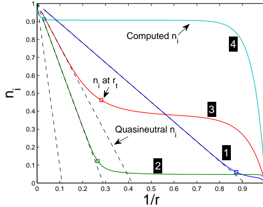
Figure 3: Computed ion density profiles for a strongly biased probe with \tau = 1 , using the following physical parameters: (1) \lambda_{De} = 0.01 , \phi_p = -10 ; we compute r_s = 1.098 and r_t = 1.14 . (2) \lambda_{De} = 0.1 , \phi_p = -100 ; we compute r_s = 3.45 and r_t = 3.77 . (3) \lambda_{De} = 1 , \phi_p = -10 ; we compute r_s = 2.40 and r_t = 3.57 . (4) \lambda_{De} = 100 , \phi_p = -20 ; we compute r_s = 9.13 and r_t = 32.28 . The dashed lines are the quasineutral solutions (Eq. (20)), and the squares indicate the densities at r_t . For each case r_t is obtained from r_s by solving Eq. (25), r_s being the intersection point of the quasineutral solution with the n_i = 0 line. Computations have been performed with the KE equations, but CE calculations would be indistinguishable with such negative \phi_p .
