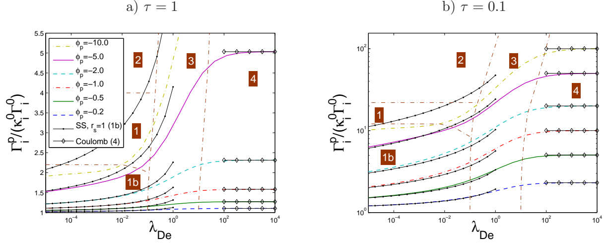
Figure 4: Evolution of the collected ion flux \Gamma_i^p (normalized to \tilde{\Gamma}_i^0 = \kappa_i^0 \Gamma_i^0 = N_\infty D_i / R_p ) with \lambda_{De} in CE plasmas, for \tau = 1 (a) and \tau = 0.1 (b). “SS, r_s = 1 ” curves correspond to Eq. (37), and “Coulomb” asymptotes to Eq. (40). The \Gamma_i^p - \lambda_{De} space is divided in four regions corresponding to the regimes described in Tab. 1. Region “(1b)” is a subsection of region (1) with 1 \leq r_s \leq 1.1 .
