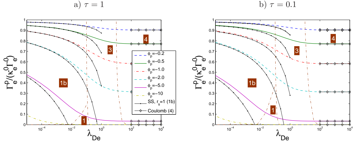
Figure 5: Evolution of the collected electron flux \Gamma_e^p (normalized to \tilde{\Gamma}_e^0 = \kappa_e^0 \Gamma_e^0 = N_\infty D_e / R_p ) with \lambda_{De} in CE plasmas, for \tau = 1 (a) and \tau = 0.1 (b). “SS, r_s = 1 ” curves correspond to Eq. (38), and “Coulomb” asymptotes to Eq. (42). The \Gamma_e^p - \lambda_{De} space is divided as in Fig. (4).
