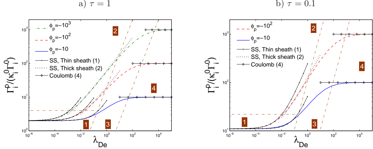
Figure 7: Evolution of the ion flux density (normalized to \tilde{\Gamma}_i^0 = \kappa_i^0 \Gamma_i^0 = N_\infty D_i / R_p ) with the electron Debye length for \tau = 1 (a) and \tau = 0.1 (b), in the strong bias regime. The \Gamma_i^p - \lambda_{De} space is divided in four regions corresponding to the regimes described in Tab. 1. “SS, Thin sheath” (region 1) and “SS, Thick sheath” (region 2) curves correspond to Eq. (47) with r_s respectively given by Eq. (46) and Eqs (50,51). “Coulomb” (region 4) asymptotes correspond to Eq. (40).
