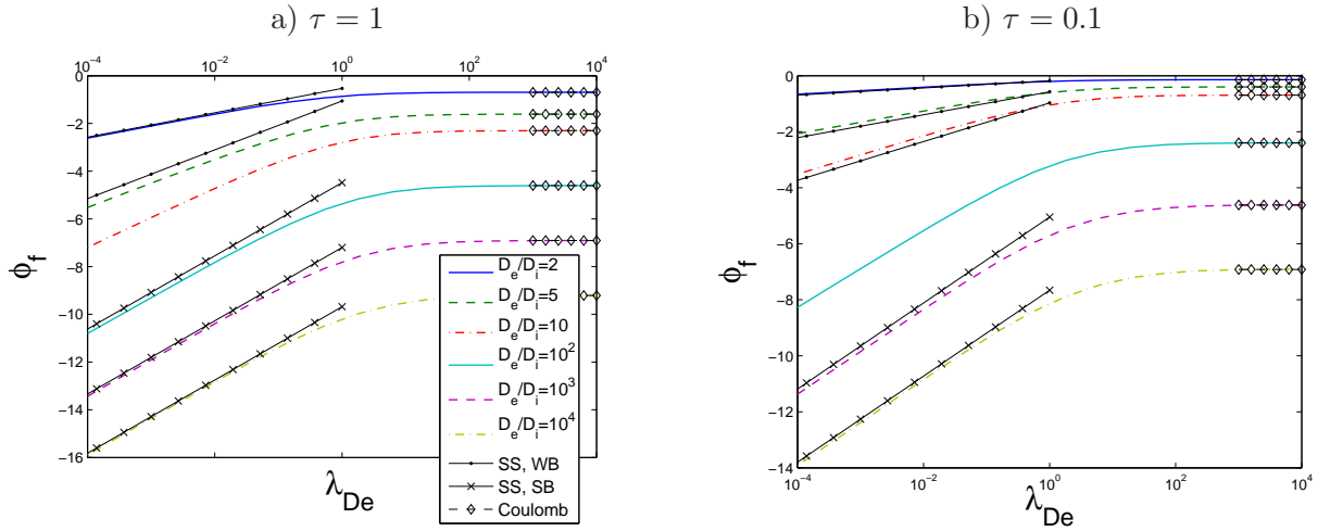
Figure 9: Probe floating potential in CE plasmas as a function of \lambda_{De} for \tau = 1 (a) and \tau = 0.1 (b). A wide range of diffusivity ratios is explored ( D_e/D_i \in [2 : 10^4] ). “SS, WB” curves correspond to the strong shielding, weak bias solutions (Eq. (53)), “SS, SB” curves to the strong shielding, strong bias solutions (Eq. (59)) and the “Coulomb” asymptotes to the solution of Eq. (60). When \phi_f is approximately between -5 and -10 , none of the two strong shielding formulas apply.
