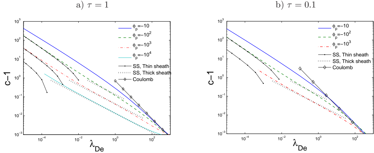
Figure 12: Dimensionless probe capacitance in CE plasmas for \tau = 1 (a) and \tau = 0.1 (b) as a function of \lambda_{De} , for \phi_p \leq -10 . “SS, Thin sheath” and “SS, Thick sheath” curves correspond to the strong shielding solutions respectively given by Eq. (74) and Eq. (75). “Coulomb” asymptotes correspond to Eq. (67).
