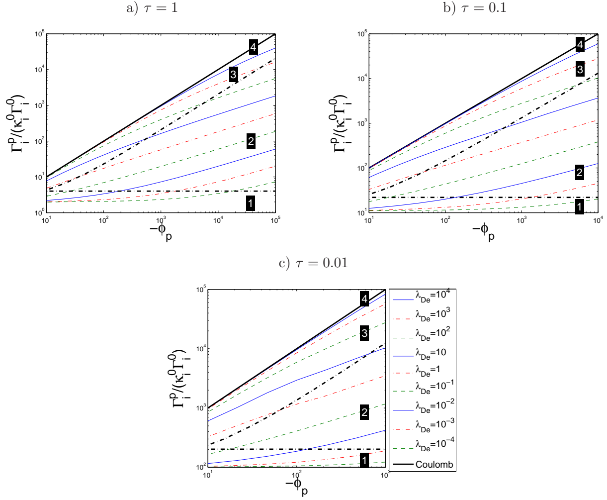
Figure 8: Current-voltage characteristics for \tau = 1 (a), \tau = 0.1 (b) and \tau = 0.01 (c), for |\phi_p| \geq 10 . The ion flux density is normalized to \tilde{\Gamma}_i^0 = \kappa_i^0 \Gamma_i^0 = N_\infty D_i / R_p . The four regions of r_s - \lambda_{De} space described in Tab. 1 are mapped to the \Gamma_i^p - \phi_p space, hence region (4) is degenerate with the “Coulomb” solution (Eq. (40)).
