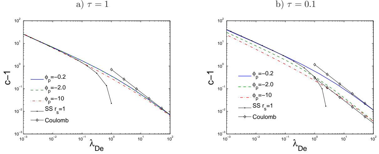
Figure 11: Dimensionless probe capacitance in CE plasmas for \tau = 1 (a) and \tau = 0.1 (b) as a function of \lambda_{De} , for \phi_p \geq -10 . “SS, r_s = 1 ” asymptotes correspond to the strong shielding solution (Eq. (72), and “Coulomb” asymptotes to Eq. (67).
