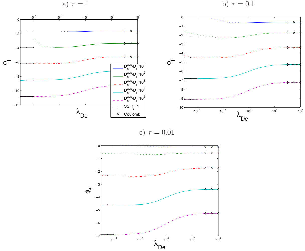
Figure 10: Probe floating potential in KE plasmas as a function of \lambda_{De} for \tau = 1 (a), \tau = 0.1 (b) and \tau = 0.01 (c). A wide range of diffusivity ratios is explored ( D_e^{app}/D_i \in [10 : 10^5] ). “SS, r_s = 1 ” asymptotes correspond to Eq. (61), and “Coulomb” asymptotes to Eq. (62). Dotted portions of curves correspond to \phi_f - \lambda_{De} parameter space where the potential profiles are not monotonic, hence we can not assert the accuracy of our results.
