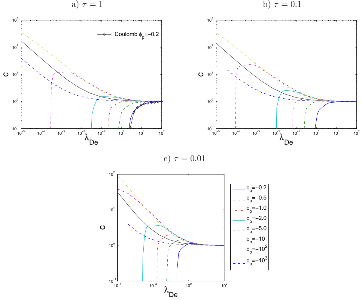
Figure 13: Dimensionless probe capacitance in KE plasmas for \tau = 1 (a), \tau = 0.1 (b) and \tau = 0.01 (c) as a function of \lambda_{De} . “Coulomb \phi_p = -0.2 ” refers to Eq. (76) with \phi_p = -0.2 .
