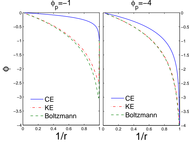
Figure 2: Potential profiles plotted against 1/r , calculated with our numerical code, for \tau = 1 , \lambda_{De} = 10^{-3} and two different biases \phi_p = -1 and \phi_p = -4 . “CE” curves are solution of Sys. (3), “KE” solution of Sys. (7) with n_e given by Eq. (11), and “Boltzmann” solution of Sys. (7) with n_e given by Eq. (10).
