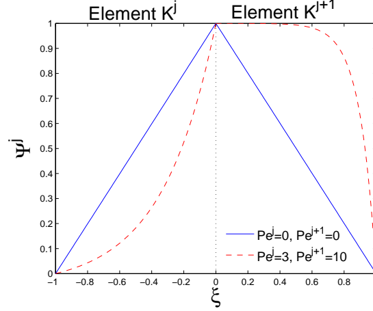
Figure 1: Example of linear ( Pe^j = Pe^{j+1} = 0 ) and exponential ( Pe^j = 3 and Pe^{j+1} = 10 ) basis functions associated with node j , with mobility going from left to right. Numerical Peclet numbers can significantly change from an element to the next if the grid is highly non-uniform.
