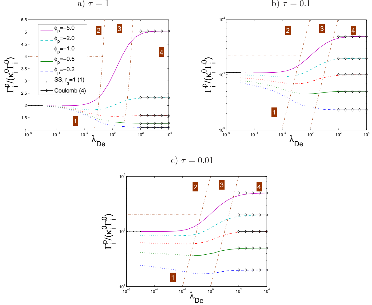
Figure 6: Evolution of the collected ion flux \Gamma_i^p (normalized to \tilde{\Gamma}_i^0 = \kappa_i^0 \Gamma_i^0 = N_\infty D_i / R_p ) with \lambda_{De} in KE plasmas, for \tau = 1 (a), \tau = 0.1 (b) and \tau = 0.01 (c). Solid lines correspond to regions of \lambda_{De} - \phi_p space where the potential profiles are monotonic (hence n_e is given by Eq. (6)). Dotted lines correspond to regions of \lambda_{De} - \phi_p space where the potential profiles have a dip below \phi_p (calculations have been performed with n_e given by Eq. (11)). “SS, r_s = 1 ” asymptotes correspond to Eq. (43), and “Coulomb” asymptotes to Eq. (40). The \Gamma_i^p - \lambda_{De} space is divided in four regions corresponding to the regimes described in Tab. 1.
