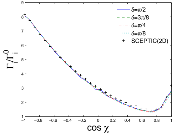
Figure 4: (a) Average ion saturation flux-density and (b) average sheath entrance potential as a function of the position projected on the drift axis ( \cos \chi ), for the case \tau = 0.1 , v_d = c_{s0} , \beta_i = 0 and a selection of \delta s. The points labeled “SCEPTIC(2D)” correspond to the solution from the appendix in Ref. [17]. SCEPTIC3D runs have been performed with r_b = 8 , n_r = 120 , n_\theta = n_\psi = 30 , and n_{\text{part}} = 51.2M .
