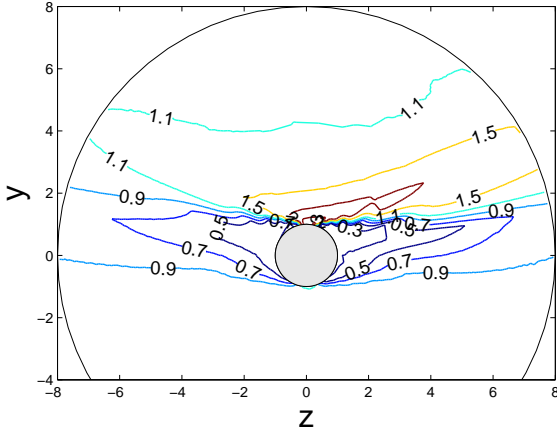
Figure 7: Contour-plots of T_{i,zz}/T_{i\infty} in the \{0, \mathbf{e}_y, \mathbf{e}_z\} -plane, with strongly magnetized ions \beta_i = 20 (except in (b) where a comparison with the magnetic-free regime is provided). (a) \tau = 1 , v_d = 0.5c_{s0} , \delta = \pi/4 and (b) \tau = 1 , v_d = 1.5c_{s0} , \delta = \pi/2 .
