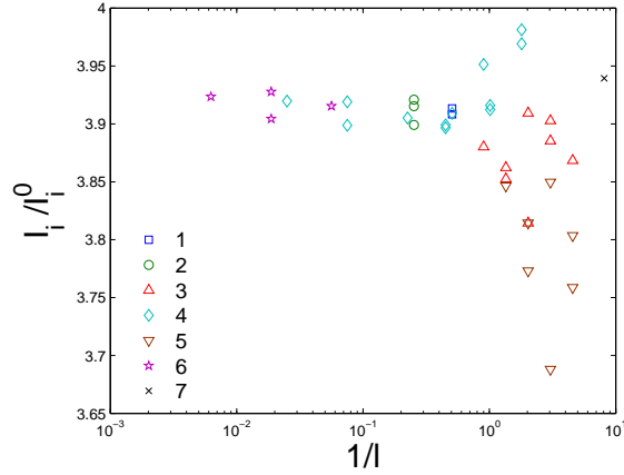
Figure 3: Ion saturation current as a function of 1/l . Each point corresponds to a different SCEPTIC3D run, where l is varied by changing the number of operating processors n_{\text{proc}} (400k particles per processor) and the grid. (1 \square ): n_{\text{proc}} = 512 , r_b = 8 , n_r = 120 , n_{\theta,\psi} = 30 . (2 \circ ): n_{\text{proc}} = 512 , r_b = 8 , n_r = 120 , n_{\theta,\psi} \leq 30 . (3 \triangle ): n_{\text{proc}} = 128 , r_b = 8 , n_r \geq 80 , n_{\theta,\psi} \geq 30 . (4 \diamond ): n_{\text{proc}} = 128 , r_b = 8 , n_r \geq 80 , n_{\theta,\psi} \leq 30 . (5 \nabla ): n_{\text{proc}} = 128 , r_b = 12 , n_r \geq 80 , n_{\theta,\psi} \geq 30 . (6 \star ): n_{\text{proc}} = 128 , r_b = 8 , n_r = 40 , n_{\theta,\psi} \leq 15 . (7 \times ): n_{\text{proc}} = 32 , r_b = 8 , n_r = 80 , n_{\theta,\psi} = 30 .
