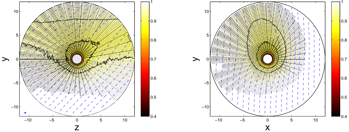
Figure 8: Charge-density contour-plots in the (a) \{0, \mathbf{e}_y, \mathbf{e}_z\} -plane and (b) \{0, \mathbf{e}_x, \mathbf{e}_y\} -plane, with plasma parameters \tau = 0.1 , v_d = 0.2c_{s0} , \delta = \pi/4 , \beta_i = 0.5 . The asymmetry in (b) is due to finite Larmor radius effects. Iso-density contours are full black, while fluid stream lines are dashed blue.
