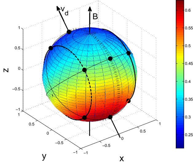
Figure 12: Three dimensional view of the probe surface, color-plotted according to the normalized ion saturation flux-density \Gamma_i/(N_\infty c_{sI}) for the plasma parameters \tau = 0.3 , v_d = 0.5c_{s0} , \delta = \pi/4 and \beta_i = 2 . The dotted, solid and dashed circles respectively correspond to cross sections located at x = 0, 1/\sqrt{3}, -1/\sqrt{3} , and the thick dots to the points where Mach probe measurements are to be made (i.e. \tan \eta = \pm 1 ).
