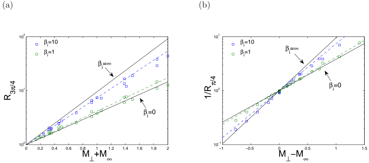
Figure 13: Upstream to downstream flux ratio on the probe major cross-section at (a) \eta = 3\pi/4 and (b) \eta = \pi/4 , versus respectively M_{\perp} + M_{\infty} and M_{\perp} - M_{\infty} , from a large set of SCEPTIC3D runs spanning v_d \in [0 : 2]c_{s0} and \delta \in [\pi/8 : \pi/2] , for a temperature ratio \tau = 1 . Also shown are the corresponding fitting lines, whose slopes 1/M_c are taken from Fig. (14a).
