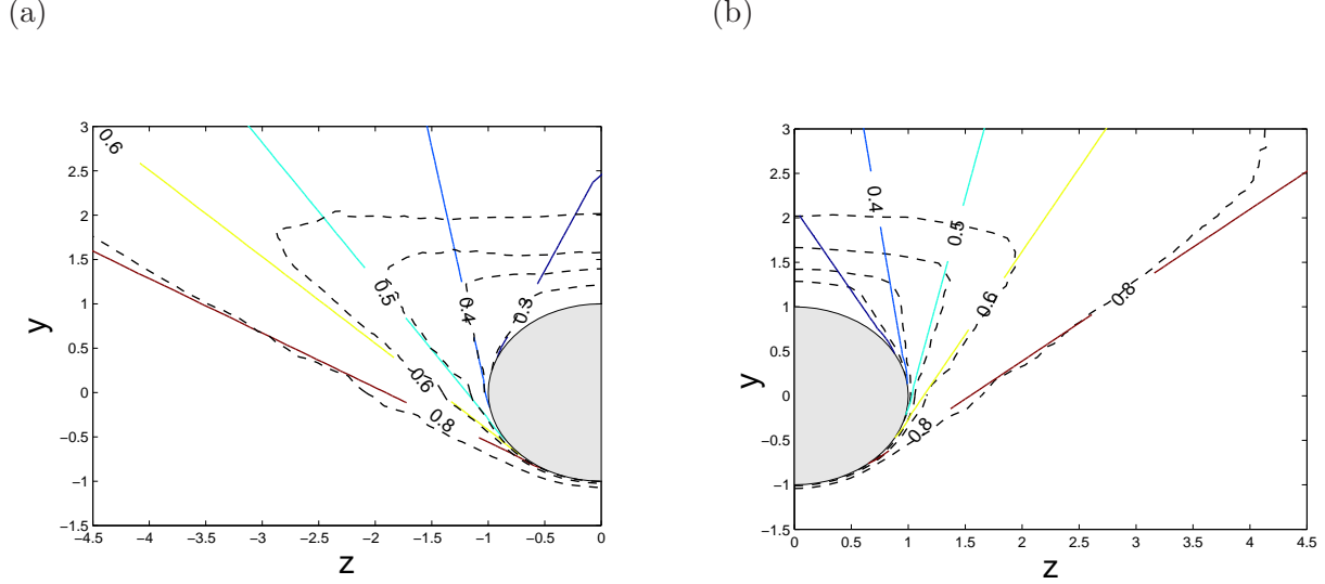
Figure 6: Comparison of density contour-lines computed by SCEPTIC3D in the \{0, \mathbf{e}_y, \mathbf{e}_z\} -plane (dashed black) with independent one-dimensional calculations (solid coloured) valid in the probe magnetic shadow when \beta_i \gg 1 . Contours are for n = 0.8, 0.6, 0.5, 0.4, 0.3 . SCEPTIC3D runs are performed with \beta_i = 20 , \delta = \pi/2 , and (a) \tau = 0.1 , v_d = 0.5c_{s0} and (b) \tau = 1 , v_d = c_{s0} . One-dimensional calculations refer to (a) the isothermal formulation [15] and (b) the kinetic formulation [16].
