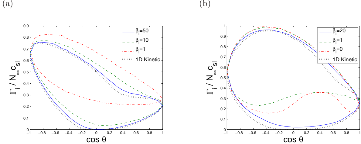
Figure 11: Angular ion flux-density distribution to the probe major cross-section in the plane of flow and magnetic field \{0, \mathbf{e}_y, \mathbf{e}_z\} normalized to N_\infty c_s I , self-consistently calculated with SCEPTIC3D for different ion magnetizations \beta_i . “1D Kinetic” refers to the semi-analytic solution of Ref. [16]. (a) \tau = 1 , v_d = c_{s0} and \delta = \pi/4 . (b) \tau = 0.1 , v_d = c_{s0} and \delta = 3\pi/8 .
