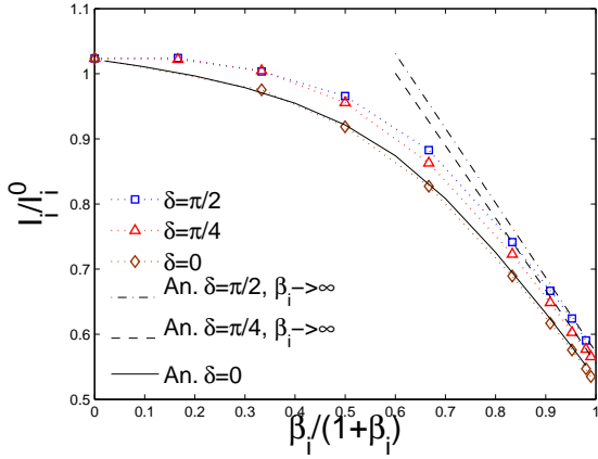
Figure 9: Total ion saturation current normalized to I_i^0 = 4\pi R_p^2 N_\infty v_{ti} / 2\sqrt{\pi} as a function of ion magnetization \beta_i in the free-flight regime (i.e. disregarding probe-induced electric field effects on the ions), computed by SCEPTIC3D for different angles of flow and magnetic field \delta . “An. \delta = 0 ” refers to the semi-analytic treatment of Refs [18, 26] for which the weak field limit is given by Eq. (16). “An. \beta_i \rightarrow \infty ” refers to the high field expansion (15). (a) v_d = 0.25v_{ti} and (b) v_d = v_{ti} .
