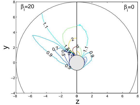
Figure 7: Contour-plots of T_{i,zz}/T_{i\infty} in the \{0, \mathbf{e}_y, \mathbf{e}_z\} -plane, with strongly magnetized ions \beta_i = 20 (except in (b) where a comparison with the magnetic-free regime is provided). (a) \tau = 1 , v_d = 0.5c_{s0} , \delta = \pi/4 and (b) \tau = 1 , v_d = 1.5c_{s0} , \delta = \pi/2 .
