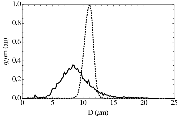
FIG. 11. Sample track diameter spectra on CR-39 detector for D^3\text{He-p} ranged down to 2.55 MeV (solid line) versus DD-p (see 2) ranged down to 2.4 MeV (dotted line). The two distributions are area normalized and plotted in arbitrary units per \mu\text{m} . The observed distribution widths are \sigma = 0.72\mu\text{m} for the DD-p versus \sigma = 2.69\mu\text{m} for the D^3\text{He-p} . This is due to broadening of the initial spectrum due to dispersion, straggling, and blooming in the filtering for D^3\text{He} as the energy loss is approximately 12 MeV. Some of the discrepancy in the mean is due to piece-to-piece CR39 variation.
