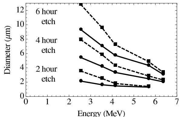
FIG. 7. Diameter of tracks observed versus energy for 2, 4, and 6 hours etch time. Solid lines represent the front CR-39 surface, dashed lines represent the back surface. Example distributions are shown in Fig. 6
