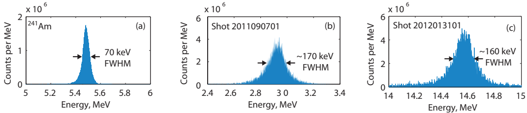
FIG. 10. Measured energy spectra for (a) an Americium-241 source (b) the LEIA DD proton source and (c) the LEIA \text{D}^3\text{He} proton source. The LEIA proton data were acquired with a 6 \mu\text{m} Al filter placed in front of the SBD. The amount of line broadening due to this filter is small ( \sim 20 \text{ keV} ) but the downshift is significant and must be taken into account for characterization of the mean proton energies. The americium source is used to infer the broadening due to the SBD, preamplifier and MCA. This instrument linewidth is then deconvolved from the measured linewidth of the fusion protons, shown here, in order to determine the linewidth of the fusion products source itself.
