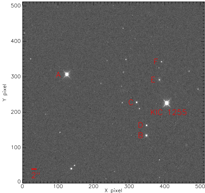
Figure 6. Full frame array of our HST /WFC3 1.4 \mu\text{m} photometry. The target star, as well as the handful of nearby reference stars (as listed in Table 2) that we perform photometry on to rule out false positive scenarios, are labeled with letters from A–F.
