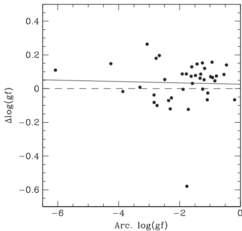
Figure 4. Comparison of \log(gf) values for all lines used in our study, with GES \log(gf) -Arcturus \log(gf) vs. Arcturus \log(gf) . The dotted line is at zero (no difference) and the solid line marks a least-squared fit to the differences. The point at \Delta\log(gf) \sim -0.6 is an Fe I line.
