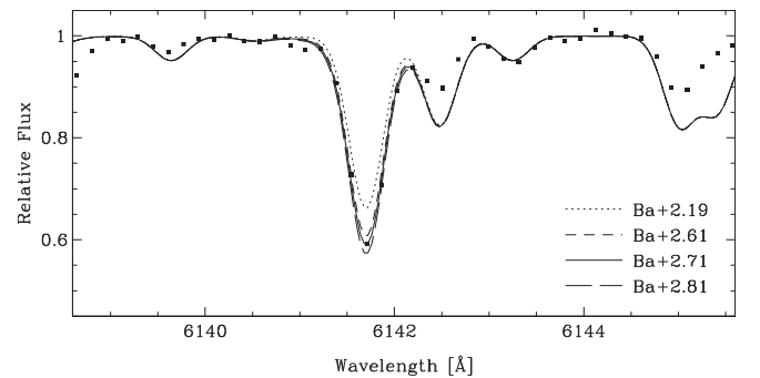
Figure 7. Comparison of the observed spectrum of star 3835 (dots) with the best spectral synthesis fit for Ba 6141 (solid line). The dashed lines indicate a typical stellar Ba uncertainty of \pm 0.10 dex, and the dotted line shows a solar [\text{Ba}/\text{Fe}] ratio for this star.
