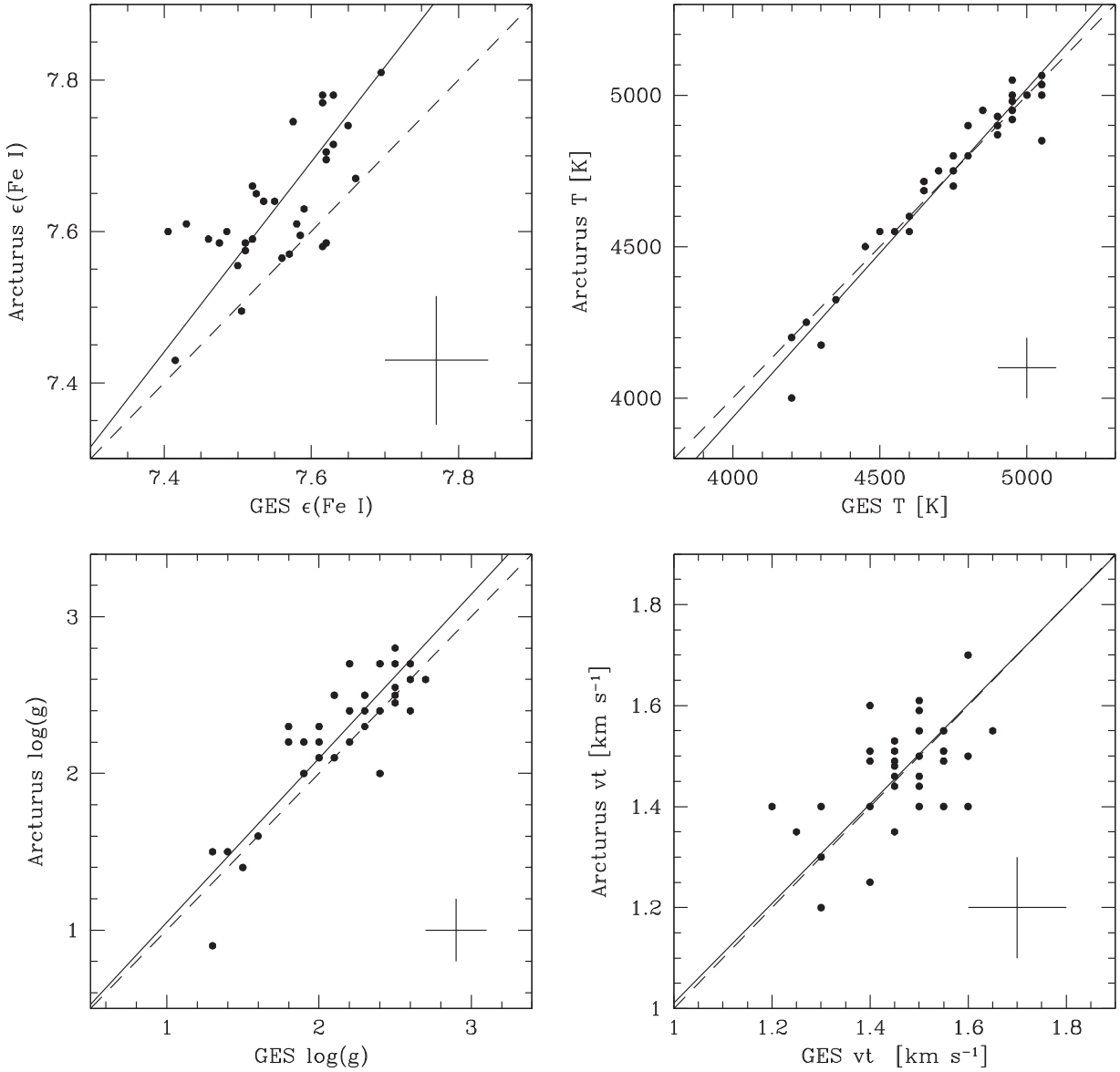
Figure 5. Comparison of atmospheric parameters spectroscopically determined using the GES linelist and Arcturus-based linelist. Dashed lines indicate a 1:1 correspondence, and solid lines are a fit to the data. Typical errors are marked on each plot.
