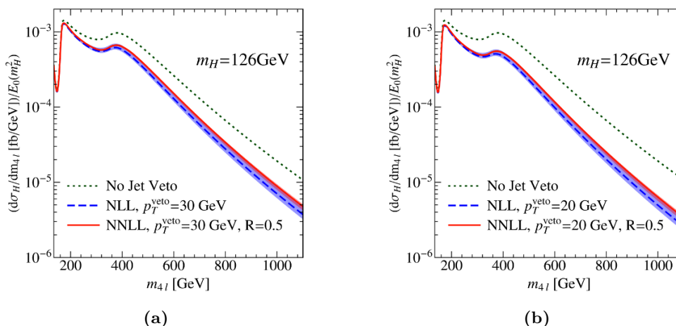
Figure 5. The off-shell Higgs cross section in the exclusive zero jet bin for p_T^{\text{veto}} = 30 \text{ GeV} in (a), and p_T^{\text{veto}} = 20 \text{ GeV} in (b), with R = 0.5 in both cases. Results are normalized by the jet veto suppression at the Higgs mass, such that the on-shell cross section is the same in all cases, allowing one to focus on the modification to the shape of the distribution. NLL and NNLL results are similar, with a small modification due to the finite jet radius, which is not present in the NLL calculation.
