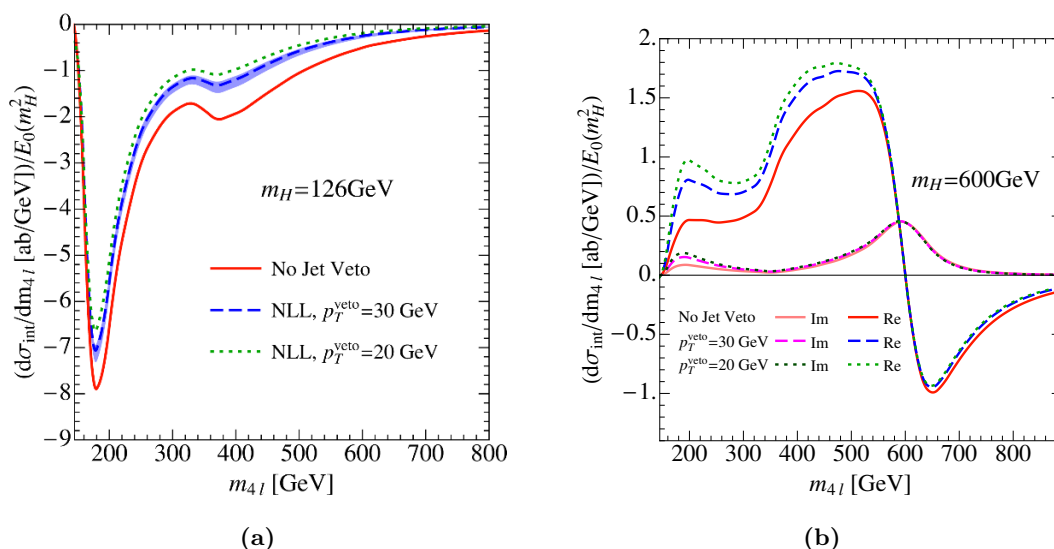
Figure 6. Signal-background interference in gg \rightarrow e^+ \nu_e \mu \bar{\nu}_\mu for (a) m_H = 126 GeV, and (b) m_H = 600 GeV. NLL predictions are shown for p_T^{\text{veto}} = 20, 30 GeV, and have been rescaled by the jet veto efficiency at m_H . The size of the signal-background interference relative to the on-shell cross section is enhanced by the jet veto for a heavy Higgs, whereas it is suppressed for a light Higgs. For m_H = 126 GeV the jet veto causes a significant reduction of the cross section in the far off-shell region relative to the on-shell cross section.
