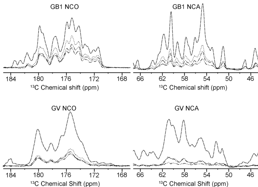
Figure 2. 1D 13 C detected comparison of 15 N- 13 C transfer methods for GB1 (top) and Gvpa (bottom) in the CO (left) and Ca regions (right). 1D 13 C CP only (dash), SPECIFIC-CP (dot), broadband DCP (dash-dot-dot), and one-bond optimized ZF-TEDOR (dash-dot). 100 kHz 1 H decoupling was used during all the 15 N- 13 C recoupling periods.
