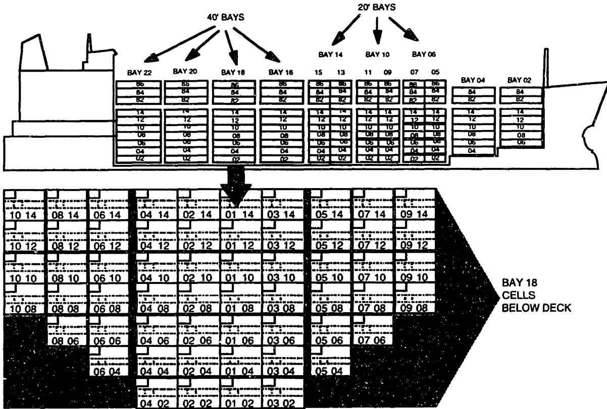
Figure 2.8 Container Stowage Addressing System
