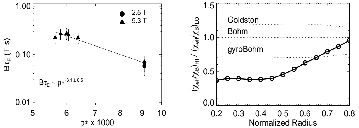
Figure 1. Results of normalized gyro-radius, \rho^* scans with q_{95} , \beta (normalized plasma pressure) and \nu^* (normalized collisionality) fixed (a) Global scaling, showing the normalized energy confinement B\tau_E vs gyro-radius, \rho^* , (b) Local scaling showing the ratios of normalized diffusivity, \chi/\chi_{Bohm} between high field (low \rho^* ) and low field (high \rho^* ) plasmas. Expectations of different types of scaling are shown by the dotted curves [5]. Both local and global analysis show approximately gyro-Bohm like scaling.
