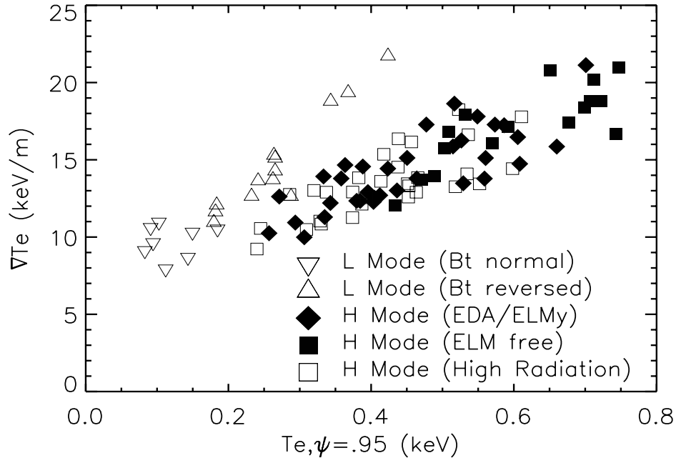
Figure 3. The average core T_e gradient is plotted vs edge temperature (measured at the 95% flux surface). The core gradient is defined as the average gradient between the outer edge of the sawtooth region and the top of the H-mode pedestal.
