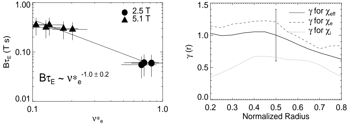
Figure 2. Results of v^* scans with q_{95} , \beta , and \rho^* fixed (a) Global scaling, showing b\tau_E vs v^* (b) Local scaling, showing the local exponent, \gamma , defined by \chi \sim \chi_{Bohm} v^{*\gamma} . Approximately linear dependence is seen in both cases.
