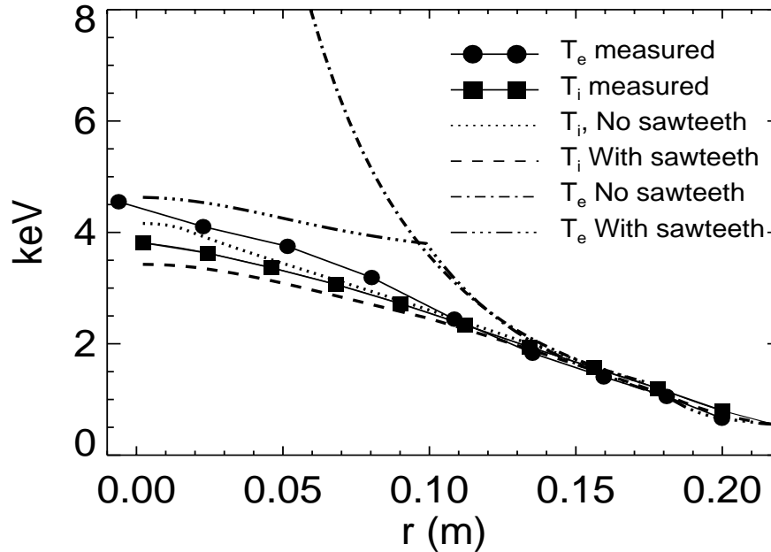
Figure 4. Comparison between experimental data and predictions of the IFS/PPPL model. Predictions both with and without an ad-hoc sawtooth model are shown. Agreement is fairly good for H-modes in C-Mod.
