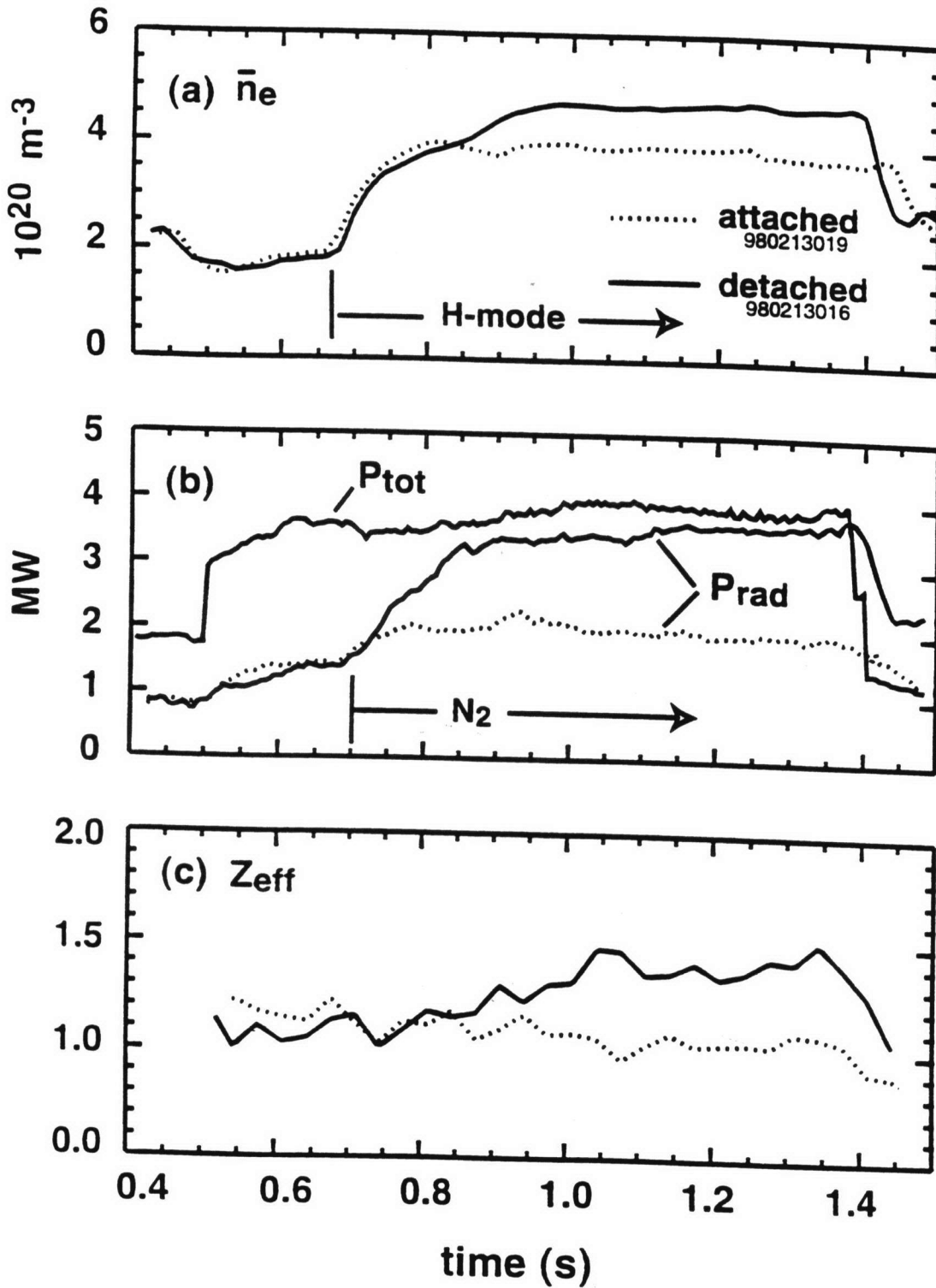
3. Some main discharge parameters for attached and detached conditions. (a) line-average density (b) power balance. P_{tot} total input power. P_{rad} total radiated power (c) central Z_{eff} .
