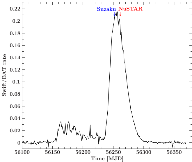
Figure 1. Swift -BAT light curve of the giant outburst of GRO J1008–57 with the NuSTAR and Suzaku observation times marked. The BAT count rate is in units of counts \text{cm}^{-2} \text{s}^{-1} .
