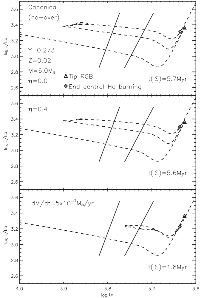
Figure 6. Same as Figure 5, but for an initial stellar mass of 6 M_{\odot} .
