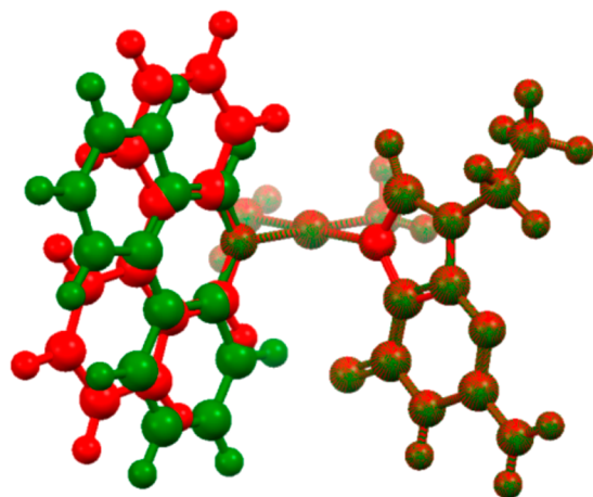
Figure 5. Overlay of the molecular mechanics optimized geometries obtained by setting the aromatic ligands perpendicular to the platinum coordination plane and rotating 180° about the platinum–phenanthridine bond.
