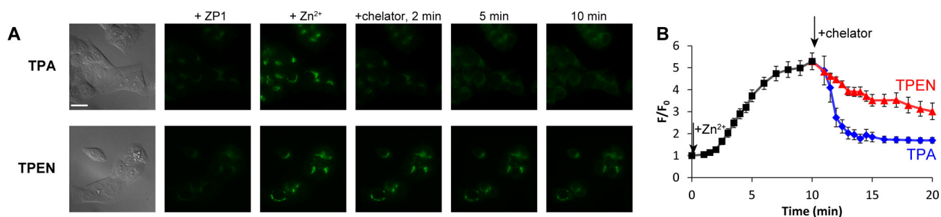
Fig. 4. (A) Fluorescence images of ZP1-treated HeLa cells. Left to right: DIC images, ZP1 signals, ZP1 fluorescence 10 min after addition of 20 \mu\text{M} zinc pyrithione, and after addition of 100 \mu\text{M} chelator (top: TPA, bottom: TPEN) recorded at 2, 5, and 10 min. Scale bar = 25 \mu\text{m} . (B) The intracellular ZP1 signals were quantitated and normalized to the levels before zinc addition. Signals from 8–12 cells in four culture dishes were averaged. Error bars represent standard errors of the mean.
