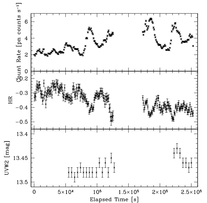
Figure 5. XMM-Newton pn and OM W2 light curves of Mkn 335 during the 2009 observation.
