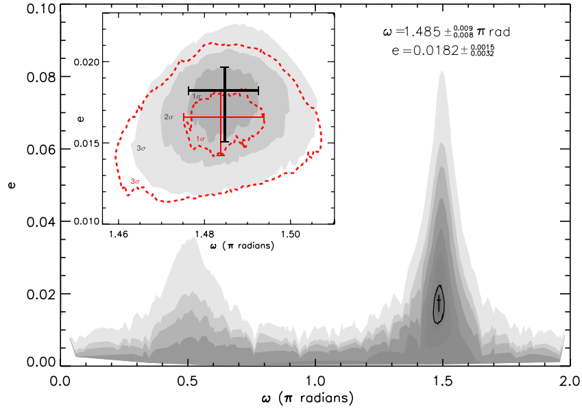
Figure 8. LC joint confidence levels for e - \omega . The LC confidence contours allow us to confirm that the values for e and \omega from the RV+LC contours are not systematically skewed by the weighting of the data, due to the abundant number of photometric data in comparison to the number of RV measurements. The figure shows the sampled parameter cross section in its entirety. The cross marks the lowest- \chi^2 point to the LC fit with 1\sigma uncertainties, surrounded by the solid line 3\sigma confidence level. The shaded contours beyond 3\sigma do not correspond to a particular uncertainty level but are shown to display the two valleys in \chi^2 when the orbit’s semimajor axis is parallel to the line of sight. The inset shows in detail the confidence interval for e and \omega within 3\sigma ; and for comparison, the dashed lines denote the 1\sigma and 3\sigma RV+LC contours from Figure 7.
