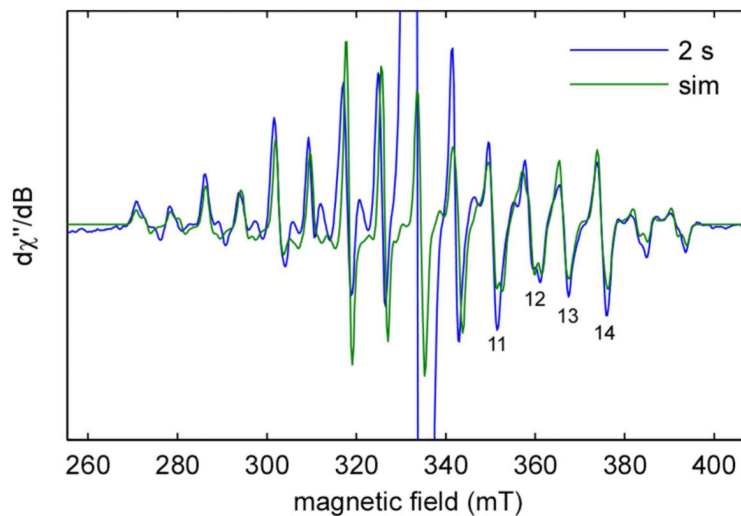
Figure 6. Simulation of the EPR spectrum of the \text{Mn}^{\text{III}}\text{Mn}^{\text{IV}} intermediate. The spectrum was obtained by subtraction of a scaled spectrum of the \text{Mn}^{\text{II}} -loaded NrdF starting material from the spectrum of the RFQ mixture of 75 \mu\text{M} NrdF, 50 \mu\text{M} NrdI, and oxygenated buffer after 2 s aging time. Simulation of the spectrum was performed as described (section 2.9). Peaks 11-14 are labeled. Spectrometer settings: temperature: 10 K; microwave frequency = 9.38 GHz; power = 20 \mu\text{W} ; modulation amplitude = 0.5 mT; modulation frequency = 100 kHz; sweep rate = 5.3 mT/s. The off-scale feature at \sim 330 mT is due to \text{NrdI}_{\text{sq}} .
