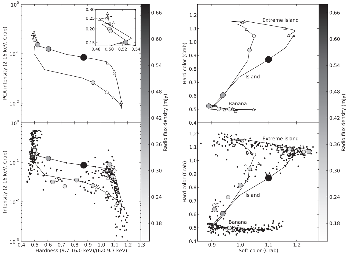
Figure 3. Left: HIDs for the 2009 November outburst of Aql X-1 (top) and all recorded outbursts with archival PCA data (bottom). Right: color–color diagrams (CCDs) for the 2009 November outburst (top) and the archival outbursts (bottom). During the 2009 outburst, the source moves anticlockwise around the HID hysteresis loop and clockwise around the CCD track (solid lines in both figures). The X-ray state at the time of the radio observations has been interpolated from X-ray observations within two days. Circles indicate radio detections at either 5 or 8.4 GHz, with the VLA, VLBA, or EVN. The size and color of the circles represent the radio flux density, according to the scale shown on the right of the plots. Open triangles denote radio upper limits. Dots show RXTE PCA measurements without simultaneous radio observations. The inset in the top HID shows a zoomed-in version of the soft state (upper left corner of the HID). Radio data from previous outbursts are taken from Tudose et al. (2009a) and Table 1. These plots show how the radio emission corresponds to the X-ray state of the source.
