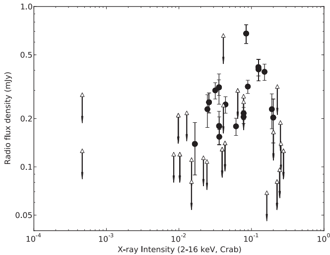
Figure 4. Correlation between radio and X-ray emission for all observations of Aql X-1, regardless of the X-ray state. Note the quenching of the radio emission at high X-ray luminosities.
