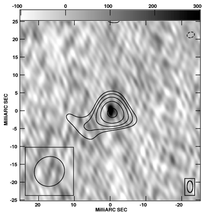
Figure 2. Gray-scale 8.4 GHz VLBA image of Aql X-1 from 2009 November 19 (MJD 55154–55155), with 5 GHz EVN contours overlaid. Contours are at levels of \pm(\sqrt{2})^n times the rms noise level of 37 \mu\text{Jy beam}^{-1} , where n = 2, 3, 4, \dots . EVN and VLBA beam sizes are shown at lower left and right, respectively. Note the marginal ( \sim 3\sigma ) extension to the southeast in the EVN image. No corresponding extension is seen with the VLBA.
