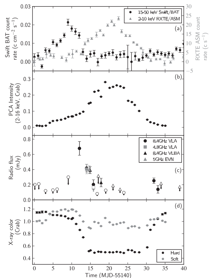
Figure 1. Radio and X-ray light curves of the 2009 November outburst of Aql X-1. (a) Swift BAT count rate ( http://swift.gsfc.nasa.gov/docs/swift/results/transients/AqlX-1_lc.txt ) in black (left-hand axis) and RXTE ASM count rate ( http://xte.mit.edu/XTE/asmlc/srcs/aqlx1.html ) in gray (right-hand axis). (b) RXTE PCA intensity. (c) Radio flux density. Circles and squares indicate VLA observations and triangles VLBI observations. Black and gray markers denote 8.4 and 5 GHz observations, respectively. Filled markers denote detections and the corresponding open markers the 3\sigma upper limits. (d) X-ray colors, defined as in Section 2.4. Note the radio detections at the state transitions where the hard X-ray color changes.
