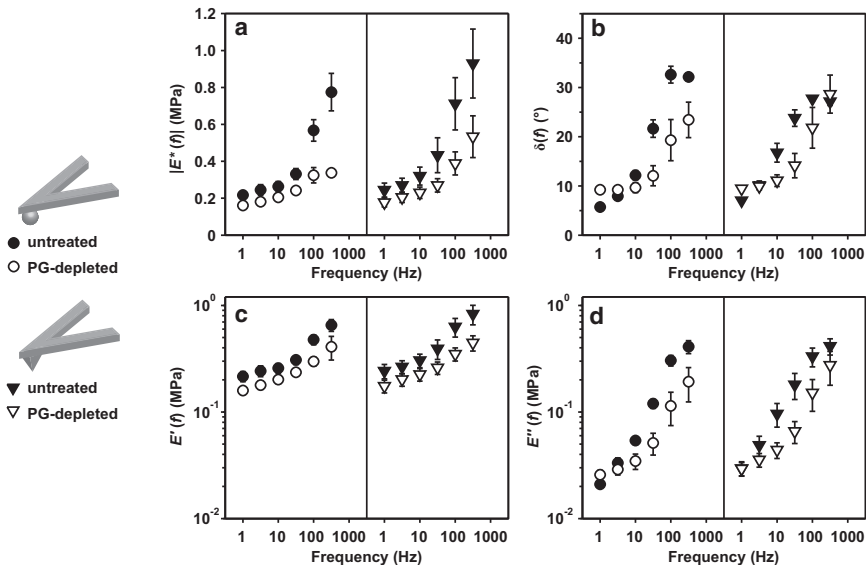
FIGURE 3 Dynamic mechanical properties |E^*(f)| (a), \delta(f) (b), E'(f) (c), and E''(f) (d) versus frequency for untreated and PG-depleted cartilage disks in PBS, using hydroxyl-functionalized spherical ( R \sim 2.5 \mu\text{m} ) and pyramidal ( R \sim 50 \text{ nm} , \alpha \sim 35^\circ ) probe tips at \sim 4 \text{ nm} z -piezo displacement amplitude ( \sim 2 \text{ nm} cartilage dynamic indentation depth amplitude), estimated using Eqs. 5–8 for n \geq 6 different locations (mean \pm SE).
