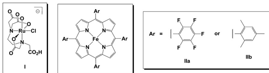
Figure 5. Model Complexes that Exhibit NOS-Type Reactivity
