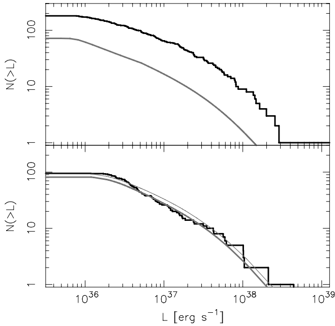
Figure 3. Upper panel: the (uncorrected) cumulative source counts within 5 arcmin from the center of Cen A, including both field and GC sources (black), compared to the expected background counts (gray) corrected for incompleteness. The sources belonging to Cen A make up the difference between the curves. Lower panel: the cumulative source counts in the 7.5–10.0 arcmin annulus (black) and the expected background (gray). About 10 LMXBs are expected in this annulus in addition to the background sources, and the thin gray line shows the expectation when these are included. The normalization of the background curves is 1.5 times the normalization given by Moretti et al. (2003).
