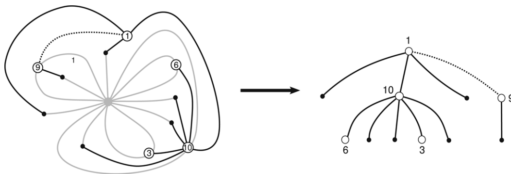
Fig. 3. From maps to trees.
