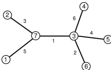
Fig. 1. The planar map corresponding to (1\ 2\ 3\ 4\ 5\ 6\ 7) = (3\ 7)(3\ 6)(2\ 7)(3\ 5)(1\ 7)(3\ 4) .
