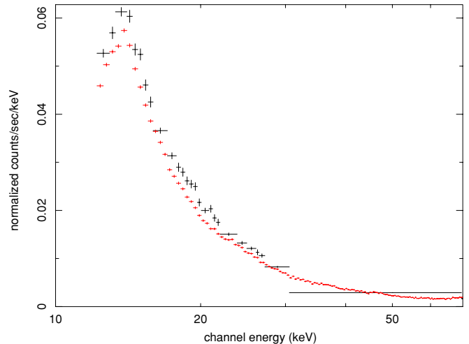
Figure 1. Suzaku HXD/PIN spectrum of 3C 33 (black) and total CXB + NXB background spectrum (red). The source spectrum has been binned to 3\sigma above the background level.
