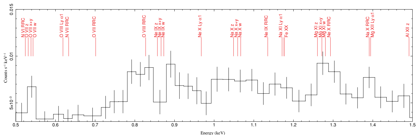
Figure 10. Combined Chandra , XMM-Newton , and Suzaku CCD spectrum of 3C 33 in the energy range 0.5–1.5 keV. Also plotted are the spectral transitions identified in the photoionized plasma of the canonical Seyfert 2 galaxy, NGC 1068.
