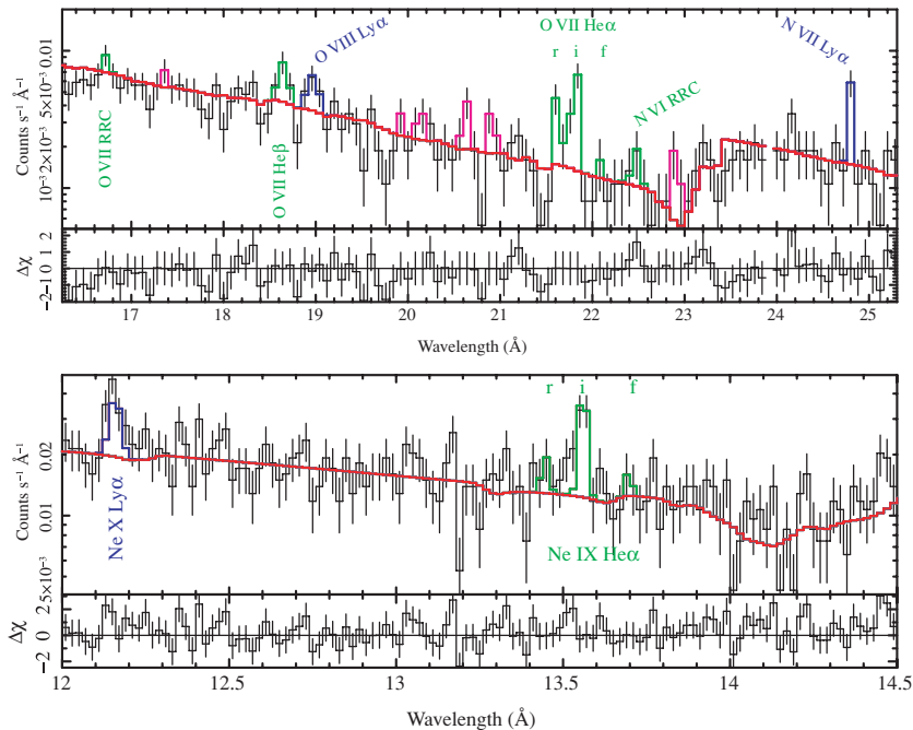
Figure 4. MEG transition-phase equivalent of Figure 3 showing data, fit, and residuals; again the red, green, blue, and magenta models correspond to the continuum, Regions I, II, and III, respectively. We have labeled the strongest lines.
