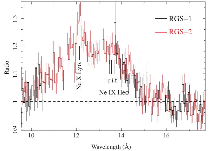
Figure 2. Data:model ratio for the RGS spectra near 12 \text{ \AA} , showing the broad bump and the location of emission features from H- and He-like Ne. The bump obscures the Ne IX lines and prevents a completely reliable determination of the Ne X line flux. In our continuum fits, we model it as a broad Gaussian with \Delta\lambda \sim 1.3 \text{ \AA} and equivalent width W_0 \sim 60 \text{ eV} .
