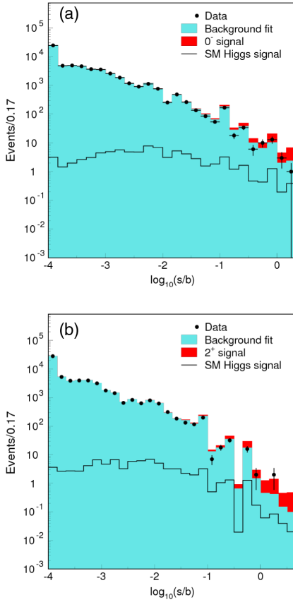
FIG. 1 (color online). Distributions of \log_{10}(s/b) for the data from all contributing Higgs boson search channels for a boson mass of 125 \text{ GeV}/c^2 for (a) the 0^- search and (b) the 2^+ search. The observed numbers of events are represented by the points, and the expected exotic signals are shown as histograms with \mu_{\text{exotic}} = 1 stacked on top of the backgrounds, which are fit to the data within their systematic uncertainties. The expected s/b ratios of the exotic signal over the background yield are used to rank analysis bins. The background predictions do not include the contributions from the SM Higgs boson, which are shown as separate histograms, not stacked. The error bars shown on the data correspond to the square root of the observed data count. Underflows and overflows are collected into the leftmost and rightmost bins, respectively.
