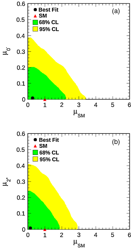
FIG. 2 (color online). Combined two-dimensional posterior density of the measured (a) 0^- -vs- 0^+ and (b) 2^+ -vs- 0^+ cross sections, normalized to the SM predictions.
