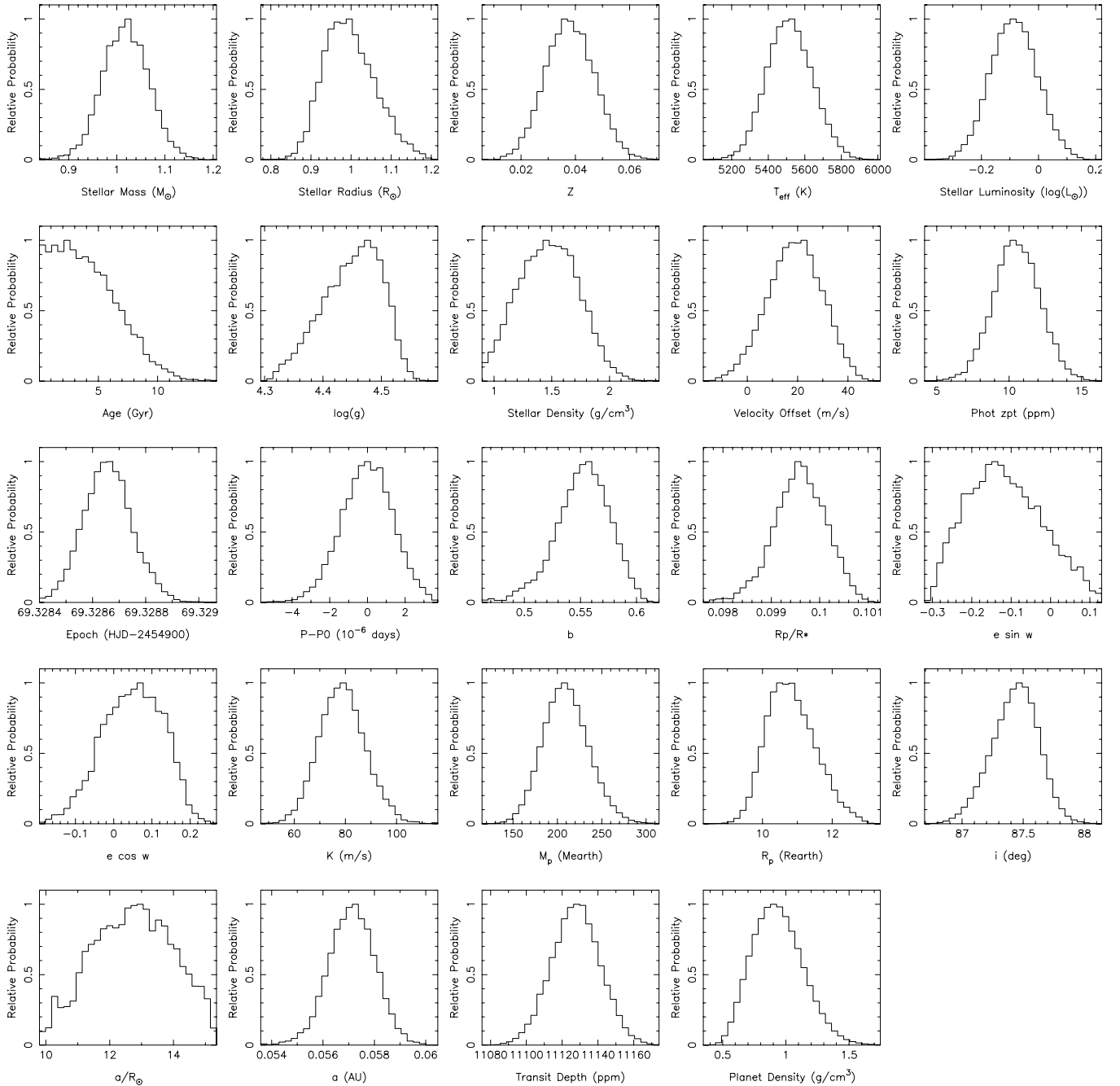
Figure 12. Markov Chain Monte Carlo distributions for the model parameters for the Kepler-15 system. The resulting values and uncertainties of the system parameters are listed in Table 4. For the period value we plot the difference to P_0 = 4.942782 days.
