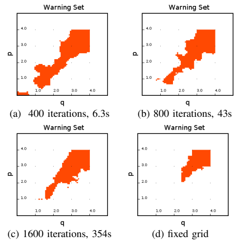
Fig. 7: Warning sets (darker, red) for semi-autonomous collision avoidance, generated by coupled-iGame. A fixed grid solution is also shown. \dot{p} = 0.75 , \dot{q} = 0.75 .
