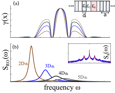
FIG. 4. (Color online) Dressed decay rate and the RO spectrum based on SALT solutions of a 1D PhC laser. (Inset) A quarter-wave PhC (period a = 1\text{mm} and alternating layers with permittivities \epsilon_1 = 16 + 0.1i and \epsilon_2 = 2 + 0.1i and thicknesses d_1 = \frac{a\sqrt{\epsilon_2}}{\sqrt{\epsilon_1 + \sqrt{\epsilon_2}}} and d_2 = a - d_1 ). The center region has permittivity \epsilon_d = 3 + 0.1i and contains gain atoms with bandwidth \gamma_{\perp} = 3\text{mm}^{-1} and resonance frequency \omega_a = 25\text{mm}^{-1} . (a) Dressed decay \gamma(\mathbf{x}) evaluated using (13) at five pump values ( 2D_{\text{th}} brown, 3D_{\text{th}} blue, 4D_{\text{th}} black, and 5D_{\text{th}} gray). (b) Side-peak spectrum S_{\text{RO}}(\omega) evaluated using (42) for the five pump values of (a). (Inset) Full simulated spectrum S_a(\omega) on a semilog scale (of base 10) of the homogeneous time-delayed model (33) with \gamma_0 = 0.09, A = 10, B = 0, R = 0.01 (in arbitrary frequency units). The noisy signal is the simulation result and the red curve is the theoretical line shape (42).
