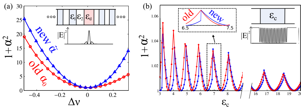
FIG. 5. (Color online) (a) The generalized (blue) and traditional (red) \alpha factors of a PhC laser vs relative detuning \Delta\nu \equiv \frac{\omega_0 - \omega_a}{\omega_0} . (Upper inset) Quarter-wave PhC geometry (see caption of Fig. 4). The gain parameters are \gamma_{\perp} = 3\text{mm}^{-1} and a varying \omega_a . (Lower inset) Intensity distribution of the lasing mode. (b) \alpha factor for an open-cavity laser vs passive permittivity \epsilon_c . Blue (red): generalized (traditional) \alpha factor. (Upper inset) Dielectric slab, of permittivity \epsilon_c , bounded by air on both sides, containing gain atoms with \omega_a = 15\text{mm}^{-1} , \gamma_{\perp} = 3\text{mm}^{-1} . (Lower inset) Intensity distribution of the lasing mode. (Leftmost inset) Enlarged segment of the main plot, around \epsilon_c = 7 .
