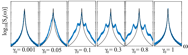
FIG. 3. (Color online) Simulated spectrum of the time-delayed model (33) with \text{Re } C = 10 and R = 0.1 (in arbitrary frequency units) at six values of \gamma_0 (using a base 10 logarithmic scale for the y axis). The noisy signal is the simulation result and the black curves are Lorentzian line shapes with widths given by (29).
