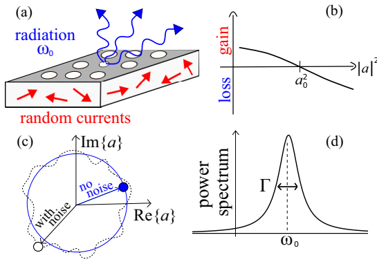
FIG. 1. (Color online) Schematics illustrating linewidth physics. (a) Photonic-crystal laser cavity [33] emitting radiation from the lasing mode at frequency \omega_0 , perturbed by random currents. (b) The squared amplitude is stabilized around a_0^2 . Below (above) a_0^2 , the medium provides light amplification (attenuation). (c) Phasor diagram for the complex field amplitude: a circular oscillation (with |a| = a_0 ) for the noise-free mode and a perturbed path for noise-driven mode. Noise drives small amplitude fluctuations and possibly large phase drifts. (d) The line shape is a Lorentzian \sim \Gamma/[(\omega - \omega_0)^2 + (\frac{1}{2}\Gamma)^2] , centered around \omega_0 with width \Gamma .
