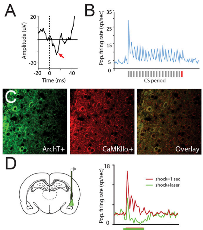
Fig. 1. Auditory CS-evoked responding in LA cells, preferential ArchT expression in LA pyramidal neurons, and optical inhibition of aversive shock-evoked responding. ( A ) Population-averaged auditory-evoked field potential response amplitude (y axis) in response to the final auditory CS pip (the time point at which the auditory stimulus will overlap with the aversive shock during subsequent training) before threat conditioning. The x axis “0” point represents the onset of the auditory stimulus. Red arrows denote the short latency portion of the response, which is known to be potentiated following fear conditioning and was used for the statistical analyses as in prior work. ( B ) Population-averaged CS-evoked firing rate responses during the preconditioning test session from single tone-responsive LA neurons ( n = 11/38 total cells) recorded in awake, behaving animals (–5 – 25 s total time period in PSTH from CS onset at first gray bar, 250-ms bins on x axis). Gray bars under the x axis denote individual auditory pips during the CS with the final pip denoted by a red bar. ( C ) ArchT ( Left ) and CaMKII \alpha ( Center ), a marker for LA pyramidal neurons, immunolabeling in LA sections. Overlaid image is shown on Right . ( D, Left ) Graphical depiction of dual optogenetic illumination and LA neural recording of shock-evoked responses. ( Right ) Population-averaged peri-event time histogram showing footshock-evoked firing rate responses (in spikes per second) in extracellularly recorded LA neurons ( n = 7 ) without (red trace) or with (green trace) overlapping laser illumination. Shock-evoked responses were significantly larger during the shock alone compared with shock + laser trials (Wilcoxon matched-pairs test: Z = 2.20 , P = 0.03 ).
