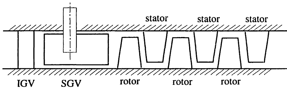
Figure 3.6: A schematic of MIT three-stage compressor with a Servo Guide Vane (SGV) between the IGV and first rotor.
