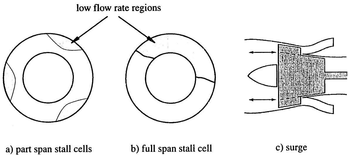
Figure 1.3: Three typical instability patterns in compression systems.
