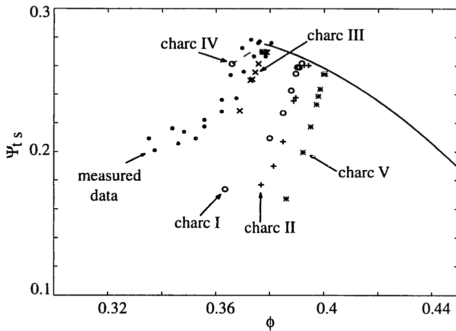
Figure 4.6: Computed results of stall characteristics for mismatched compressor with different left-side characteristics.
