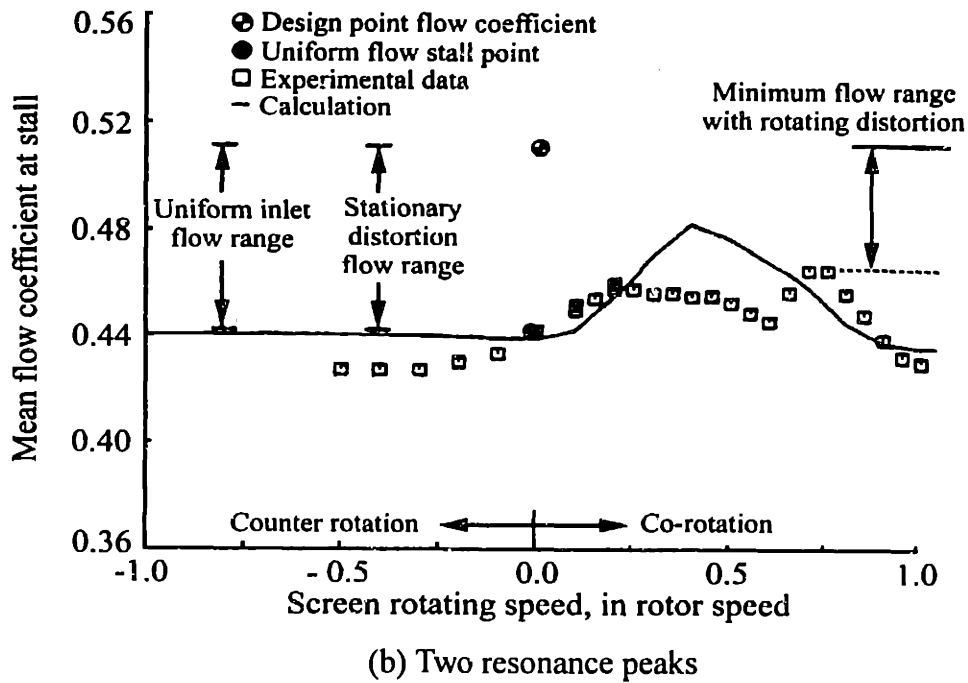
Figure 1.7: Two types of compressor resonance response to rotating inlet distortions.
