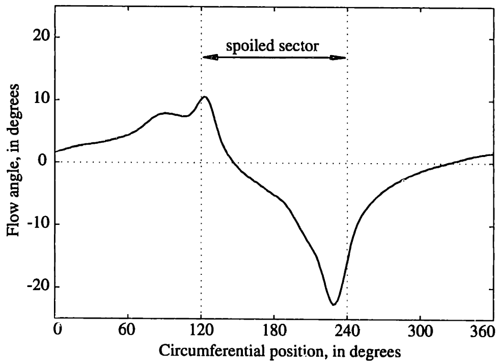
Figure 6.21: The flow angle distribution at the mid-span of the rotor inlet for Stage 35 with a total pressure distortion upstream.
