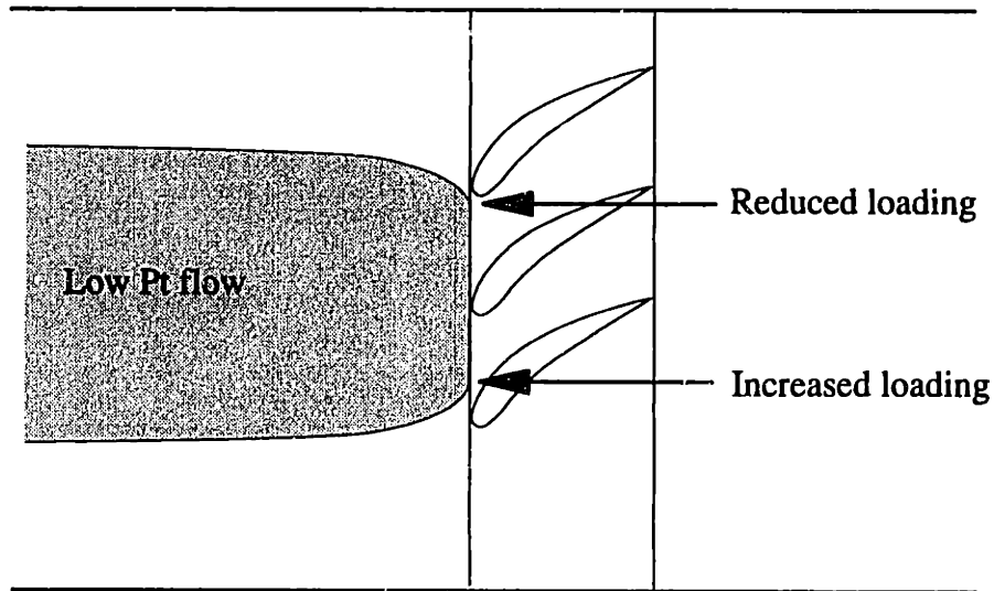
Figure 6.17: The loading on the front rotor is changed due to the induced swirl at the compressor inlet.
