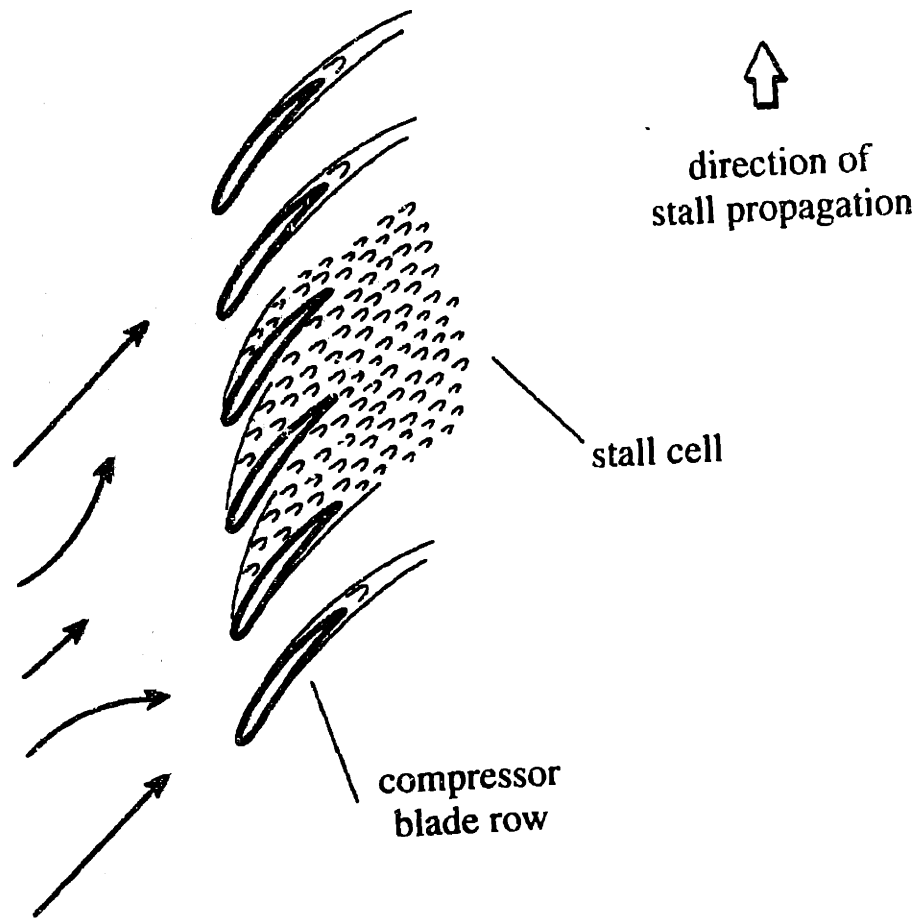
Figure 1.6: Emmons's rotating stall cell propagation mechanism.
