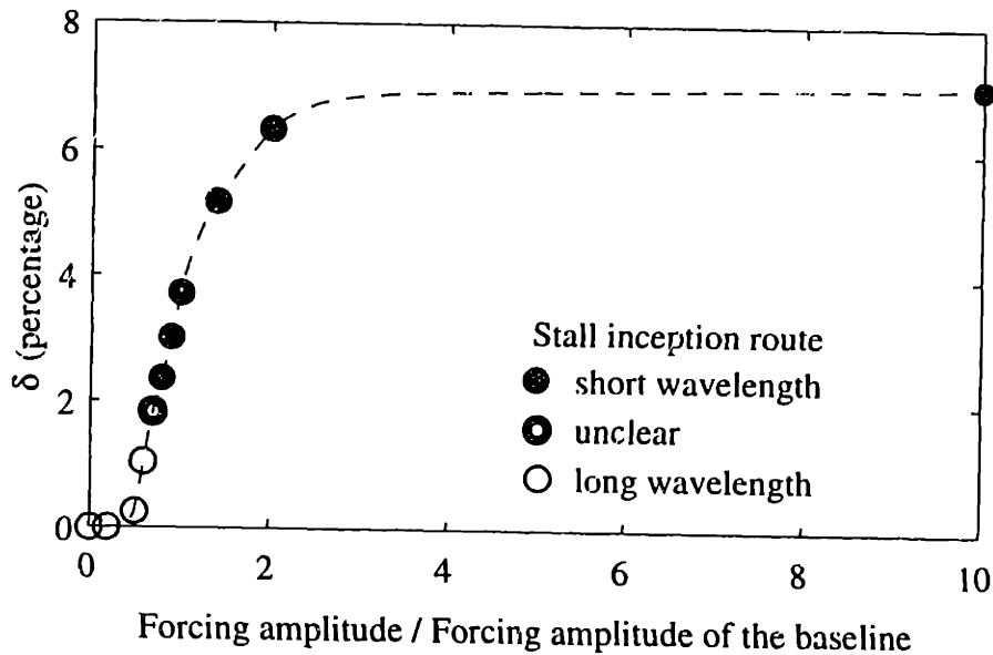
Figure 4.2: Effects of initial spike forcing amplitude on stall point and inception type.
