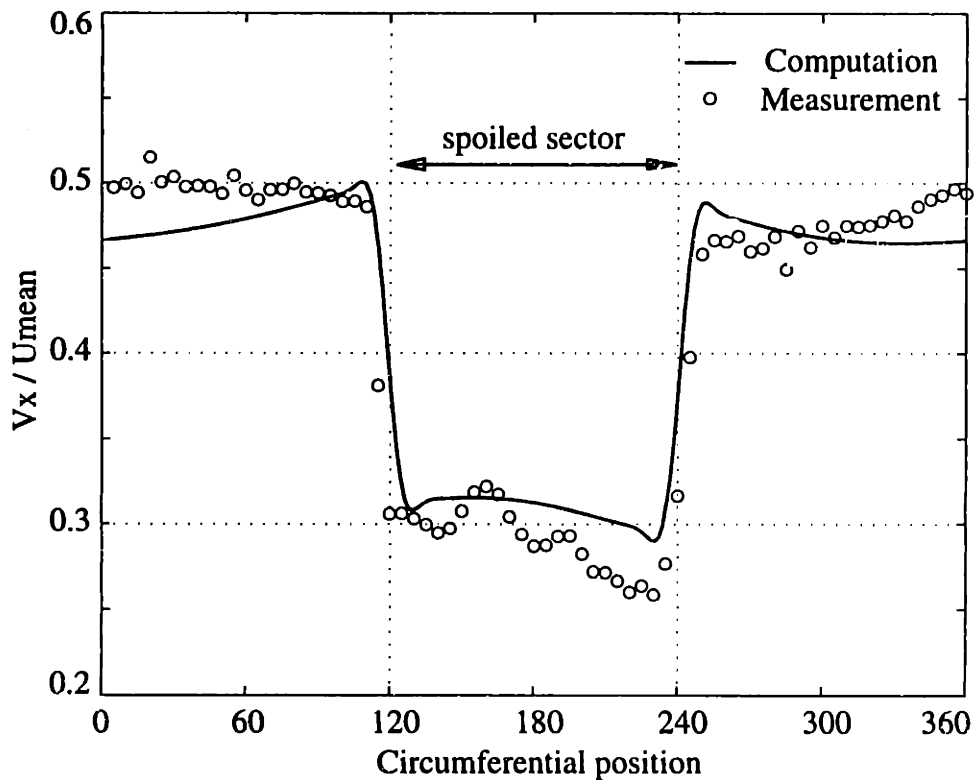
Figure 6.13: The computed and measured [65] flow coefficient at the upstream location of Stage 35.
