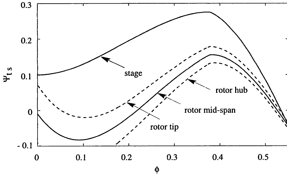
Figure 3.8: Stage characteristic of GE compressor.
