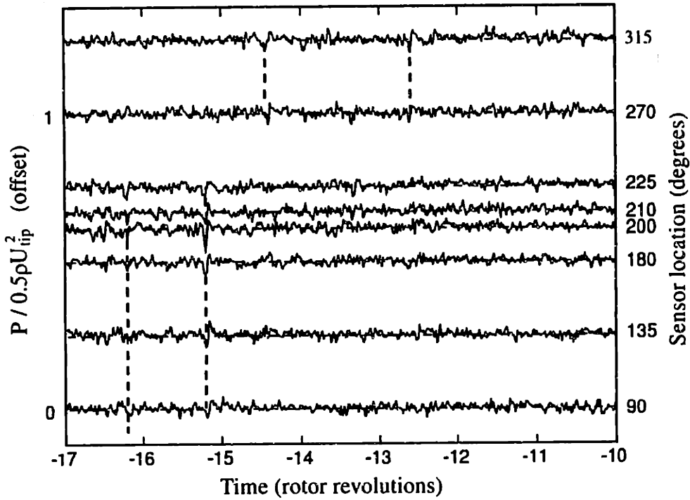
Figure 2.8: Experimental evidence of tip-spikes prior to the development of stall at t=0 . The pressure traces, from sensors at different circumferential positions at the first rotor exit, are shifted relative to first trace so that disturbances traveling at 71% of rotor speed line up vertically. Guide lines identify propagating spikes. [56]
