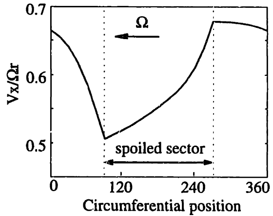
b) Hynes-Greitzer compressor
