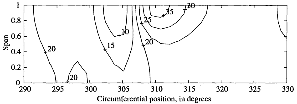
a) Tangential flow angle contours
