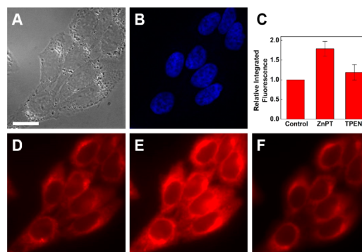
Figure 2. Fluorescence microscopy of live HeLa cells incubated with 1 \mu\text{M} ZBR4 and 10 \mu\text{M} Hoechst 33258 at 37 °C for 15 min. (A) Differential interference contrast (DIC) image. (B) Nuclear staining by Hoechst 33258. (C) Quantification of \text{Zn}^{2+} -induced fluorescence response (mean \pm SD; N = 54 ). ZBR4 signal (D) before addition of exogenous \text{Zn}^{2+} , (E) 5 min after treatment with 50 \mu\text{M} ZnPT, and (F) 5 min after addition of 50 \mu\text{M} TPEN. Scale bar = 15 \mu\text{m} .
