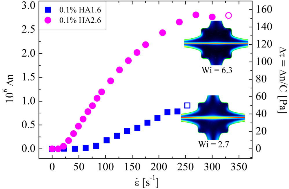
FIG. 10. Evolution of birefringence and stress as a function of the imposed strain rate in the OSCER for 0.1 wt % HA solutions. The open symbols represent the last measurements made before the onset of instability. Up until the onset of flow instabilities the device can be used as a planar extensional rheometer for complex fluids.
