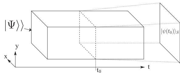
FIG. 1. Pictorial representation of the global state |\Psi\rangle . The Hilbert space of the system \mathcal{H}_S is represented by the x, y axes, the time Hilbert space \mathcal{H}_T by the horizontal axis. The state of the system |\psi(t_0)\rangle_S at time t_0 of the conventional formulation of quantum mechanics (dashed lines) is obtained by conditioning |\Psi\rangle to having time t_0 .
