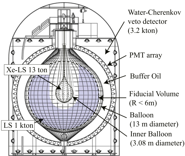
Figure 1. Schematic diagram of the KamLAND detector. The shaded region in the liquid scintillator indicates the volume for the \bar{\nu}_e analysis after the IB installation.
