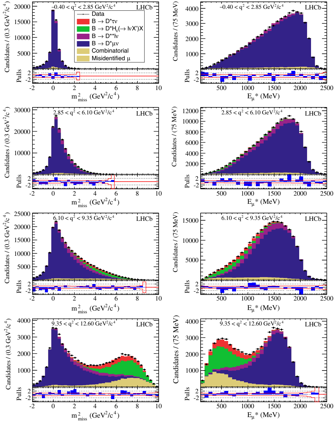
FIG. 1 (color online). Distributions of m_{\text{miss}}^2 (left) and E_{\mu}^* (right) of the four q^2 bins of the signal data, overlaid with projections of the fit model with all normalization and shape parameters at their best-fit values. Below each panel differences between the data and fit are shown, normalized by the Poisson uncertainty in the data. The bands give the 1\sigma template uncertainties.
