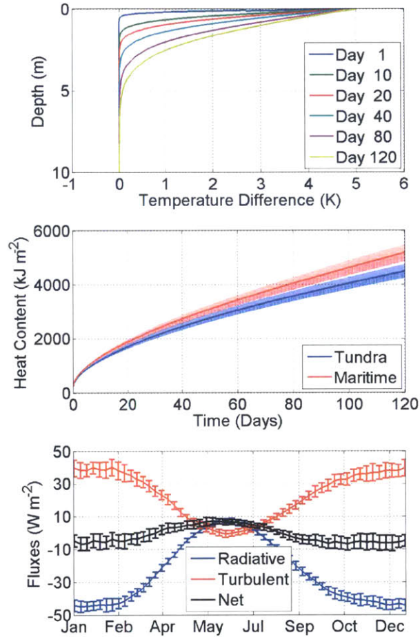
Figure 2-13: (a) Evolution of the snow temperature difference between the eight most positive and the eight most negative PC_3 winters using the heat equation with snow density estimates for the class ‘Tundra’ in Sturm et al. [2010]. (b) Additional heat content in the eight most positive PC_3 winters relative to the eight most negative PC_3 winters for the snow classes ‘Tundra’ and ‘Maritime’, which represent the most continental and the most maritime snow class respectively. The error bars are based on the estimated accuracy of the snow conductivity and density obtained from empirical relationships. (c) Mean seasonal evolution of the ERA-I heat fluxes, averaged over the most part of the ice sheet.
