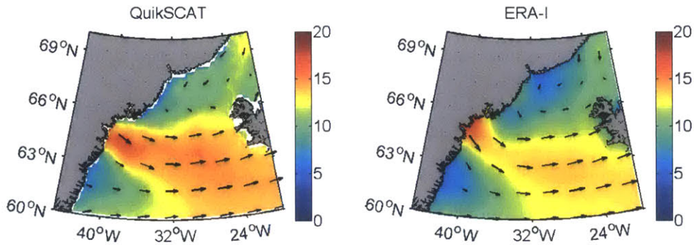
Figure 3-2: Composite of wind speed ( \text{m s}^{-1} ) during the 72 DWE that were identified with ERA-I in the time period when QuikSCAT was operating. Shown are the composites with QuikSCAT and ERA-I. The method used to identify DWE is described in section 3.4.
