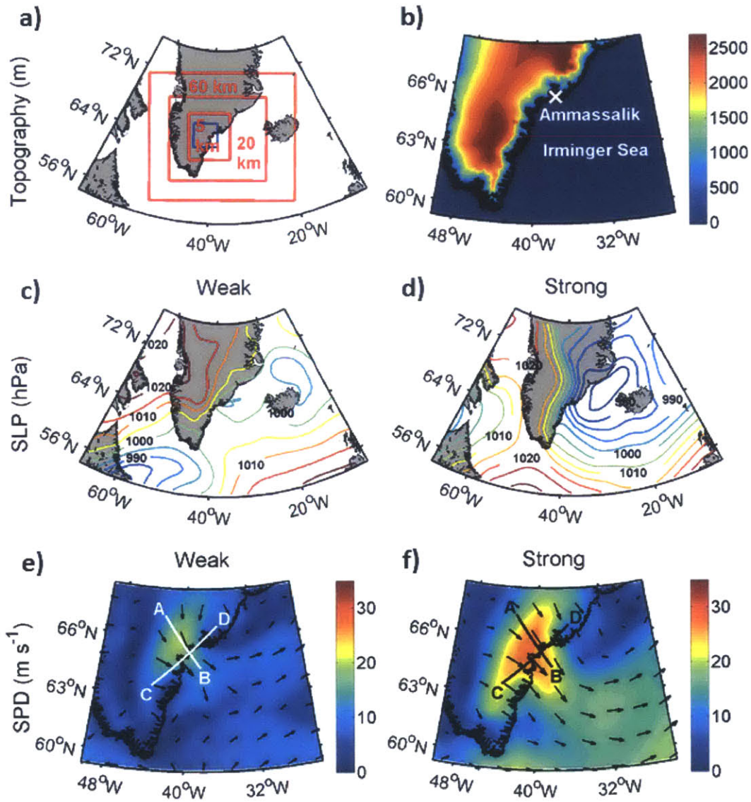
Figure 4-1: a) WRF simulation domains: The blue line delineates the 1.67 km resolution domain; b) Topography (m) in southeast Greenland including the valley of Ammassalik. The white cross indicates the location of the DMI station location; (c,d) SLP (hPa) and (e,f) wind speed ( \text{m s}^{-1} ) for the weak event in ERA-I on 9 April 2007 and the strong wind event on 3 February 1999 respectively. The lines mark the sections shown in Figures 4-3 and 4-4.
