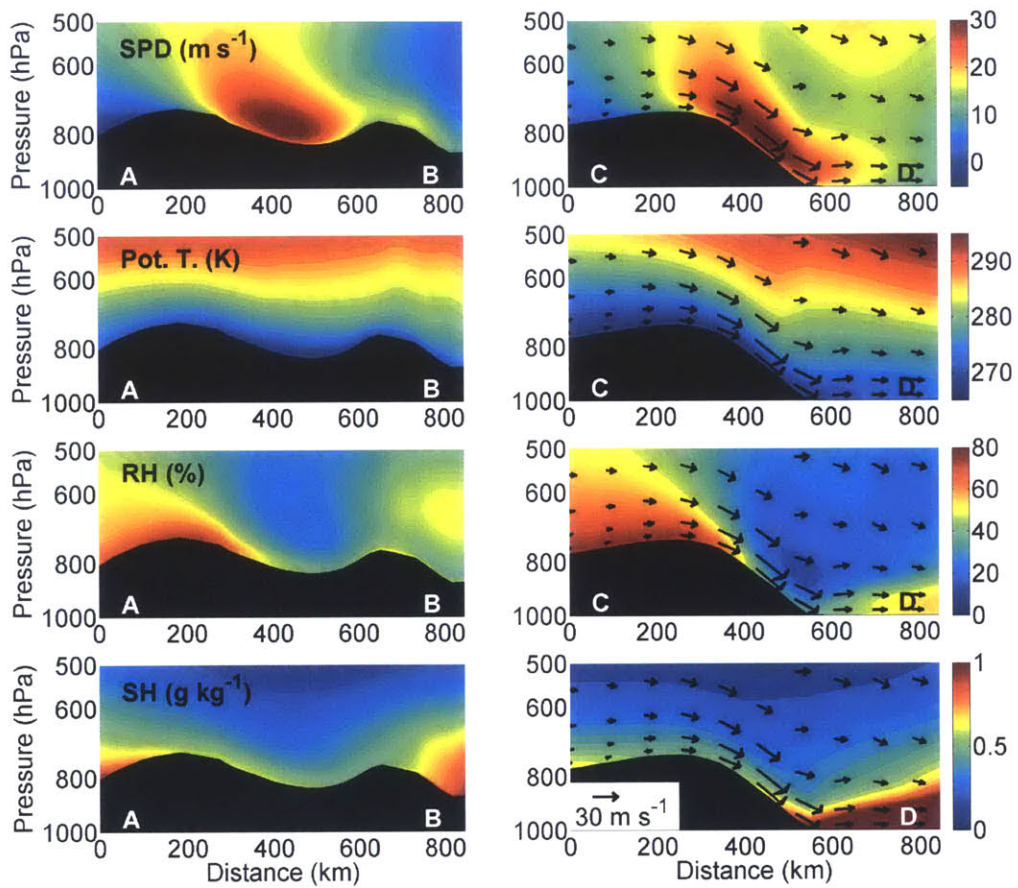
Figure 3-7: Sections along and across the downslope flow obtained from ERA-I. The section end points AB and CD are shown in Figure 3-6. The winds follow the topography closely. They are dry and cold but become moister and warmer as they cross the coastline.
