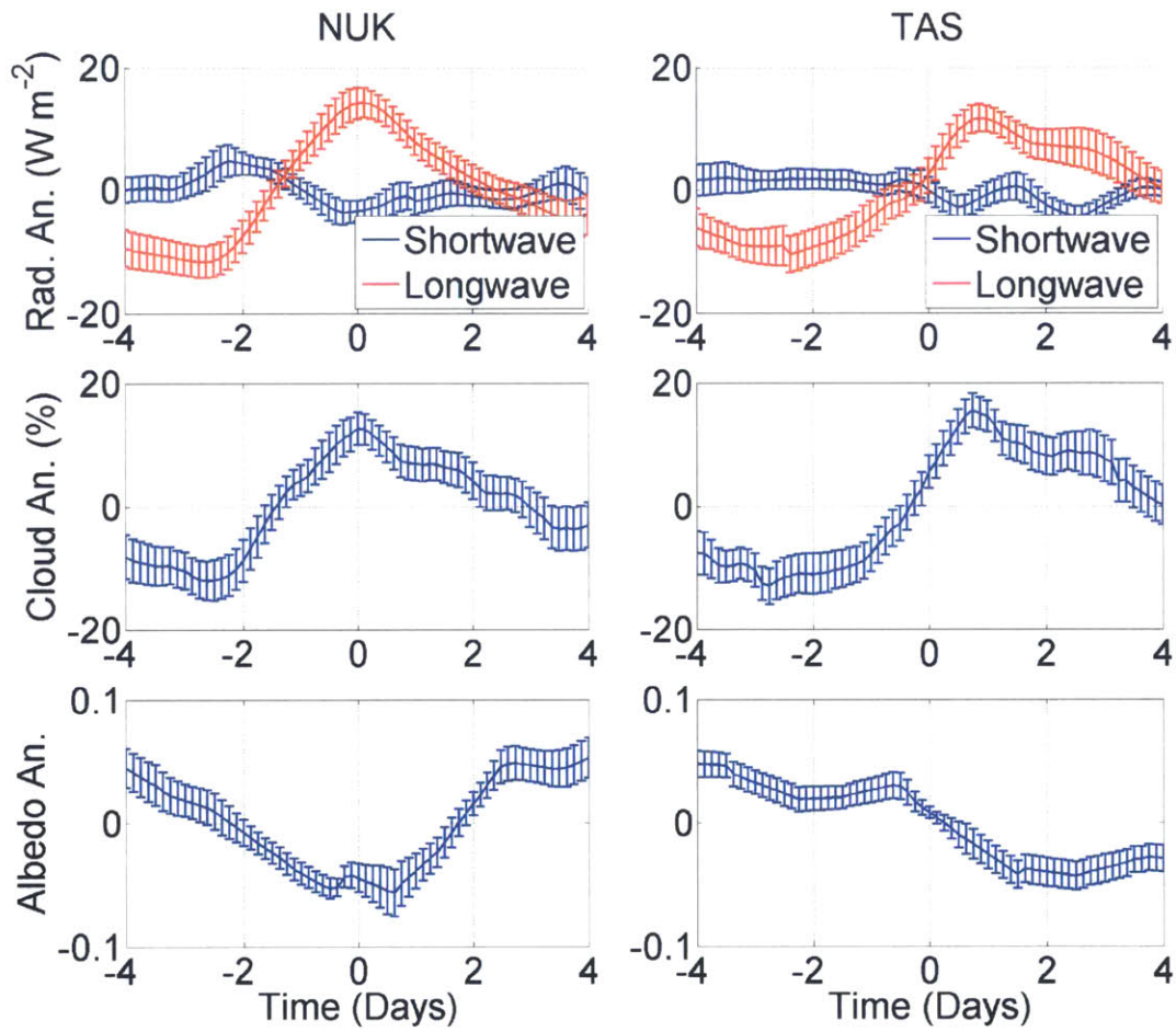
Figure 2-16: Composites of radiation, cloud cover, and albedo evolution during melt events (means subtracted) with PROMICE weather stations in Nuuk (NUK) and Tasiilaq (TAS). Both stations record \sim 60 events.
