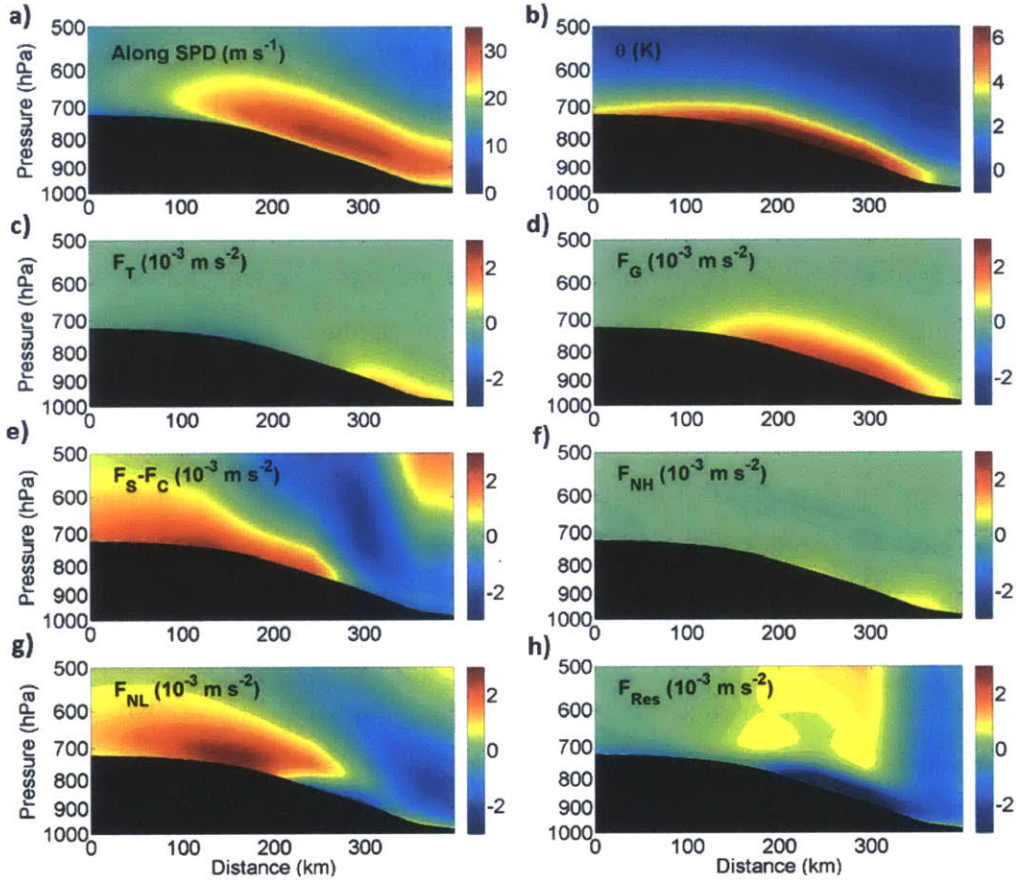
Figure 3-9: Composite analysis of the momentum balance during DWE in ERA-I along the section shown in Figure 3-8. (a) Flow component along the section. (b) Temperature deficit of the boundary layer with respect to the ambient atmosphere; a positive temperature perturbation indicates that the air is colder than that of the ambient atmosphere. (c), (d) and (e) show the thermal force F_T , the gravitational force F_G and the ambient pressure gradient force with the Coriolis force subtracted F_S - F_C . (f) The force resulting from non-hydrostatic effects F_{NH} is small compared to the ambient and gravitational force, indicating that it plays a minor role during the events, and that the splitting of the total pressure gradient is reasonable. (g) and (h) show the nonlinear advection and the residual which likely results from friction and some parametrized gravity wave drag.
