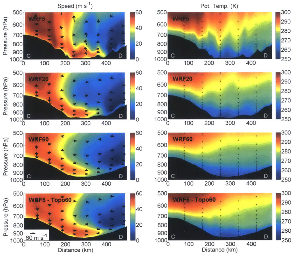
Figure 4-3: Comparison of the flow field and potential temperature in the 5 km (WRF5), 20 km (WRF20) and 60 km resolution domains (WRF60) across the section CD in Figure 4-1. The filled contours show the component of the flow across the section whereas the arrows represent the flow along this cross section. Only a few arrows are shown. The reference arrow is representative of the horizontal direction only. The vertical direction is rescaled according to the axis limits. WRF5-Topo60 indicates the case where the model resolution is 5 km and the topographic resolution is 60 km. Black crosses overlaid on the temperature field indicate the positions of the vertical model levels at selected locations across the valley.
