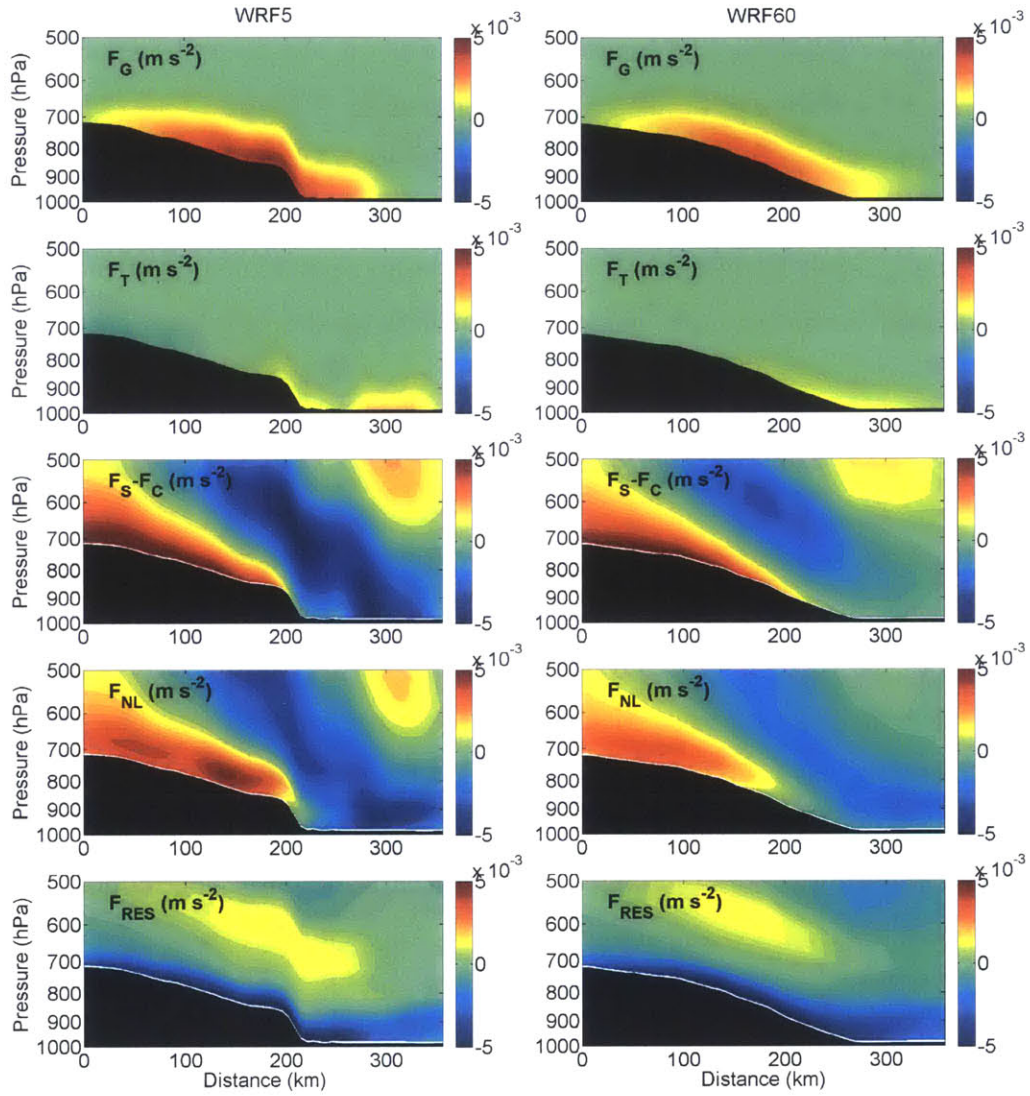
Figure 4-6: Accelerations during the strong event in WRF5 and WRF60 along the section AB shown in Figure 4-1. Shown are the gravitational acceleration F_G , thermal acceleration F_T , ambient pressure gradient and Coriolis acceleration F_S - F_C , nonlinear advection F_{NL} and the residual F_{Res} at 21:00 UTC. F_{NL} appears on the left-hand side of Equation 4.2 and is mostly balancing the pressure gradient terms. The forces are smoothed over 120 km to eliminate the small-scale variability associated with the mountain wave and to compare WRF5 and WRF60 on the same scale.
