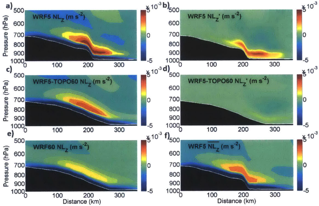
Figure 4-8: Mean and wave parts of the vertical component of the momentum flux along section AB (Figure 4-1) at 21:00 UTC. a,c,e) Total vertical momentum flux in WRF5, WRF5-Topo60 and WRF60 respectively; b,d) Wave component of the vertical momentum flux ( \overline{w^* \frac{\partial u^*}{\partial z}} ) in WRF5 and WRF5-Topo60 respectively; f) Mean component of the vertical momentum flux in WRF5 ( \overline{w \frac{\partial u}{\partial z}} ).
