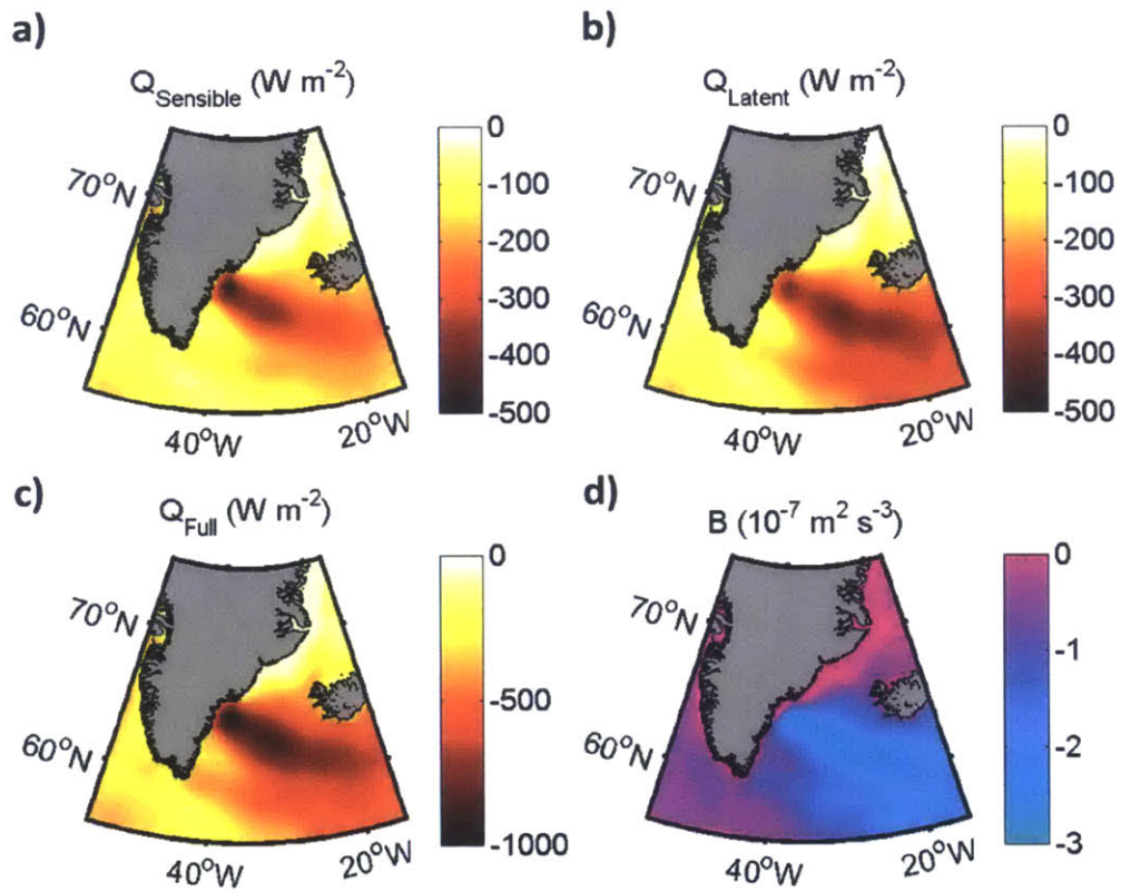
Figure 3-10: Snapshot of the sensible (a), latent (b) and total (c) heat fluxes from ERA-I for an individual DWE that occurred on 28 December 2004. The sensible and latent heat fluxes are the major contributors to the buoyancy loss (d) during this wind event.
