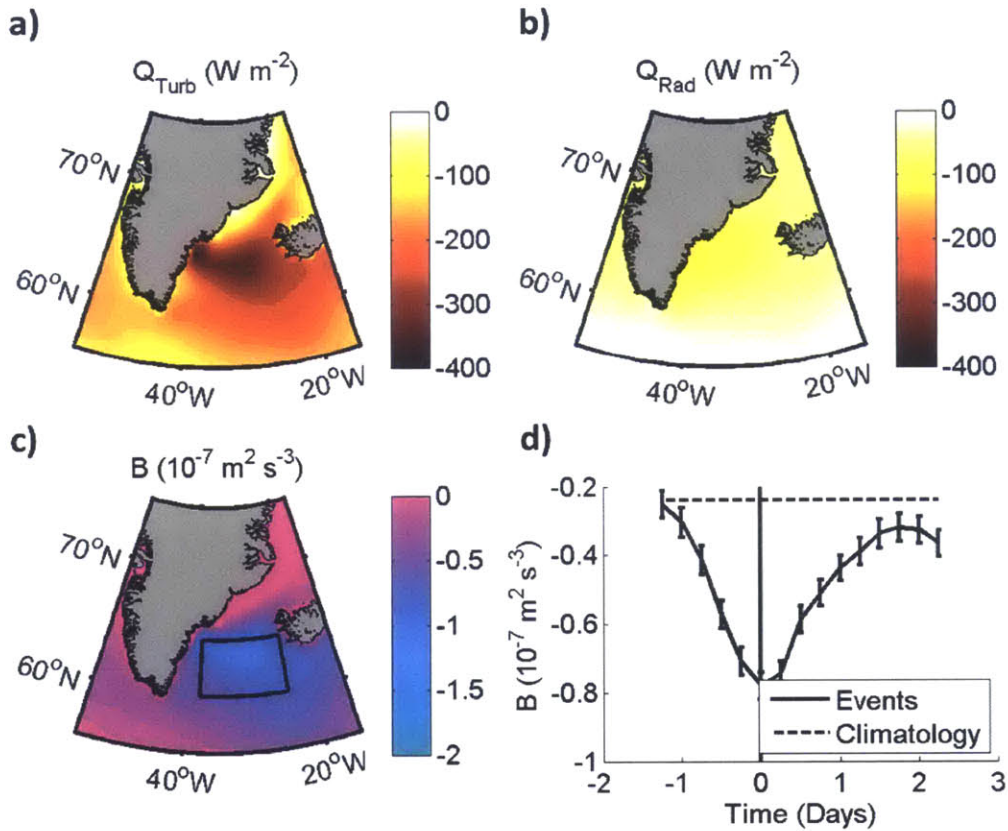
Figure 3-11: Composite of the turbulent (a) and radiative heat fluxes (b) of the wintertime (November through April) DWE. Again the turbulent heat fluxes are the major contributors to the buoyancy loss (c) of the wintertime DWE in ERA-I. (d) Composite of the ERA-I buoyancy flux evolution associated with all wintertime DWE over the Irminger Sea box shown in (c). 0 days indicates the time of the maximum wind speed. The climatological mean (November through April) is shown for reference. The duration of the enhanced buoyancy loss is almost three days.
