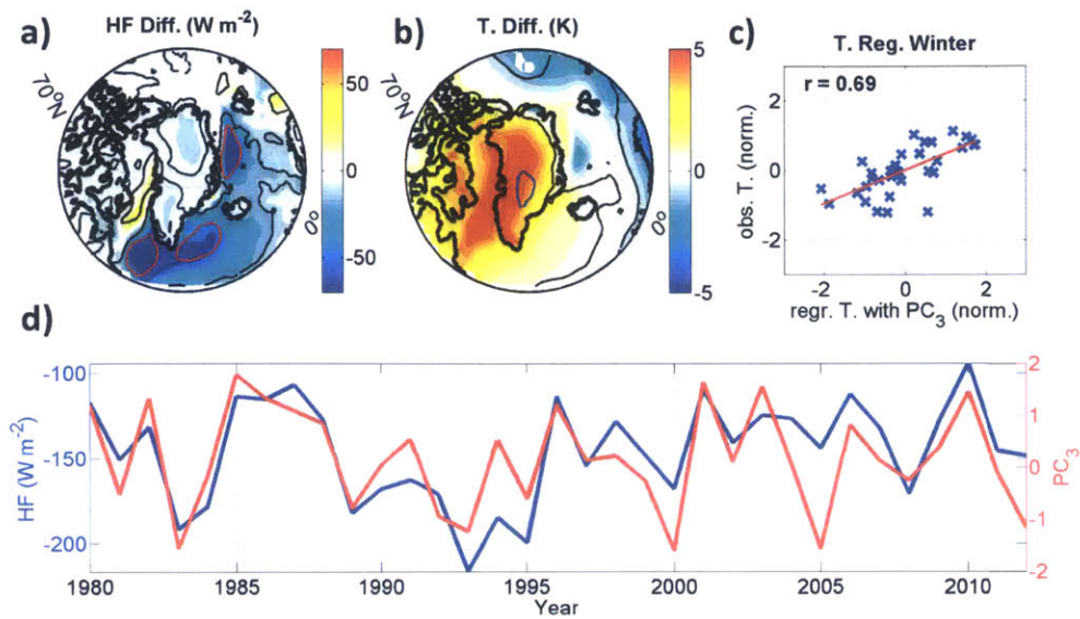
Figure 2-12: (a) Composite difference of the heat flux field ( \text{W m}^{-2} ) between the eight lowest and the eight highest \text{PC}_3 winters (DJFM) from 1979 to 2012 where \text{PC}_3 refers to the principal component of the third EOF mode (Figure 2-10). The thin black line delineates the regions in which the heat flux difference exceeds the two standard errors associated with the eight highest and the eight lowest \text{PC}_3 winters. Negative heat fluxes indicate a heat flux from the surface to the atmosphere. (b) Composite difference of the surface air temperature (K) between the eight highest and the eight lowest \text{PC}_3 winters (DJFM) from 1979 to 2012. The blue line delineates the region on which the temperature regression is based. (c) Regression of temperature variability within the region shown in (b) in winter (DJFM) using the \text{PC}_3 . (d) Inter-annual variability of the mean winter (DJFM) heat fluxes averaged over the Irminger, Labrador and Greenland Sea regions shown in (a) and the (normalized) \text{PC}_3 .
