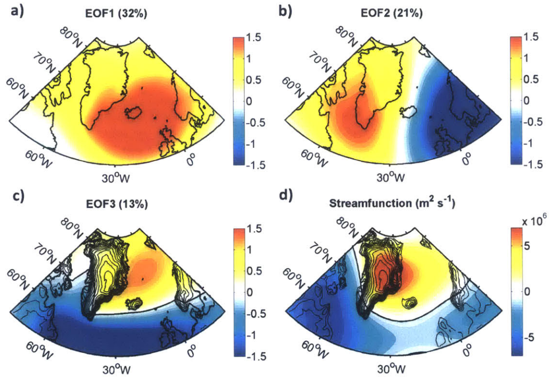
Figure 2-10: (a,b,c) EOF decomposition in ERA-I based on SLP variability from 1979 to 2012. The modes are normalized by their standard deviation, and the title indicates the percentage of the atmospheric variance that is explained by them. Topographic contours are added for the third EOF mode. The black line indicates the zero line of the third EOF mode. It runs across the top of the southern dome of Greenland. If the cyclone is north of that line, the flow across the southeast coast is northwesterly. If it is south, the flow is southeasterly. (d) Perturbation streamfunction ( \text{m}^2 \text{s}^{-2} ) derived from the topographic Rossby wave model. Despite its simplicity, the model reproduces a basic southwest-northeast asymmetry over the southeast coast, that is similar to that associated with the third EOF mode and the eastern and western wind events.
