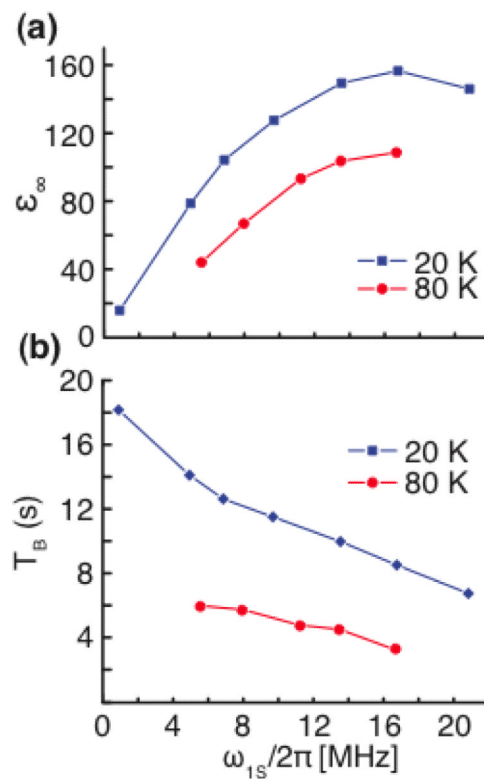
Figure 9. Microwave Field Strength and Temperature Dependence of Gd-DOTA Enhancements (a) Solid effect enhancements using Gd-DOTA at 20 K and 80 K as a function of microwave field strength. (b) Buildup times ( T_B ) at 20 K and 80 K as a function of microwave field strength.
