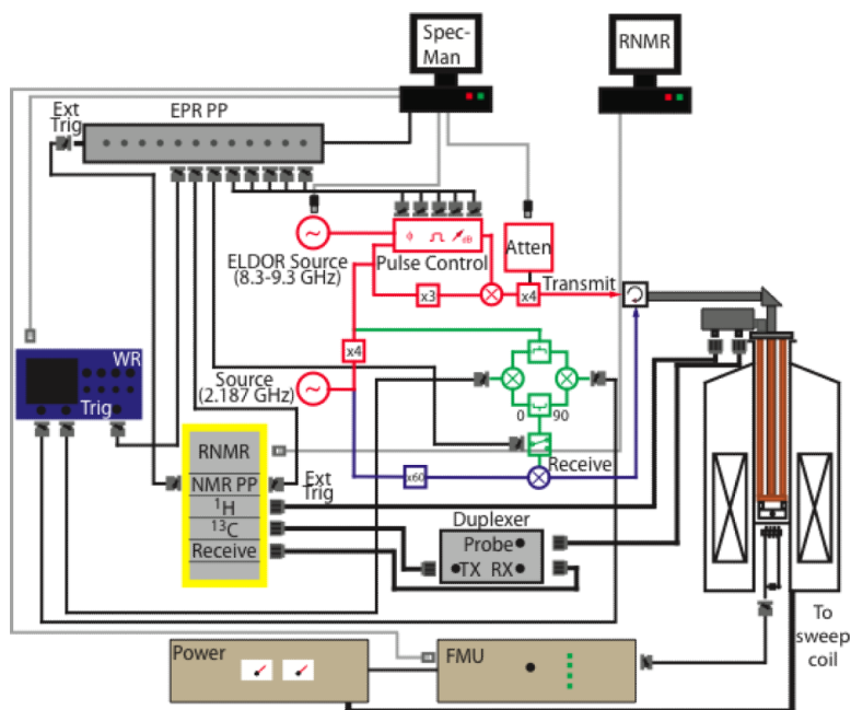
Figure 4. Full Spectrometer Configuration
