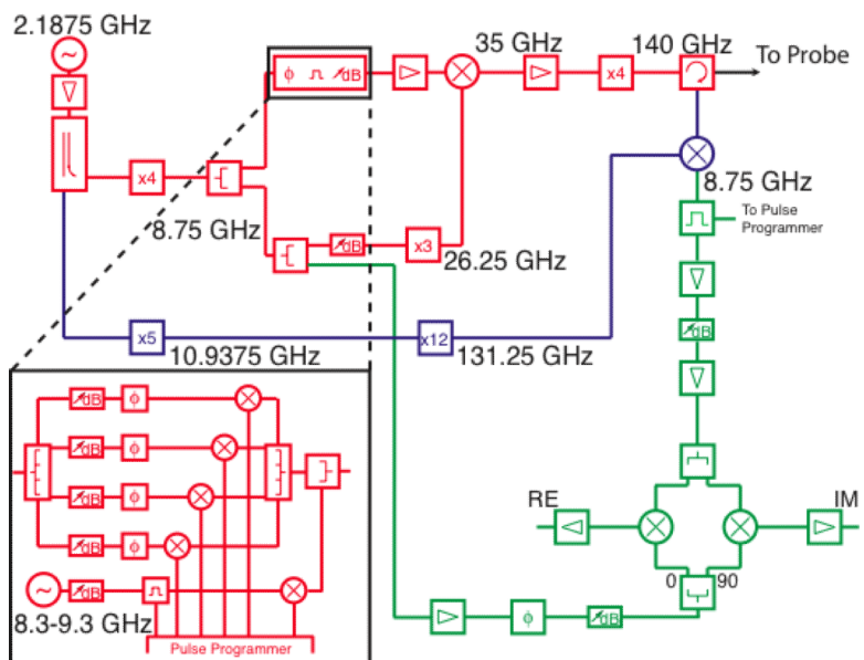
Figure 1. 140 GHz EPR Bridge Design
