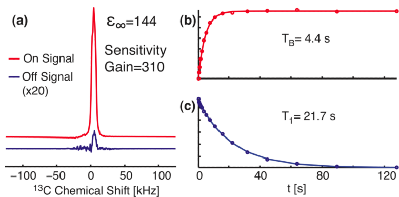
Figure 8. Solid effect DNP Sensitivity Gain
