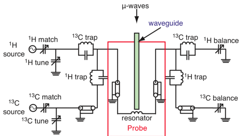
Figure 3. Balanced RF Circuit Design
