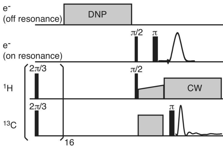
Figure 5. Simultaneous EPR and NMR Detection
