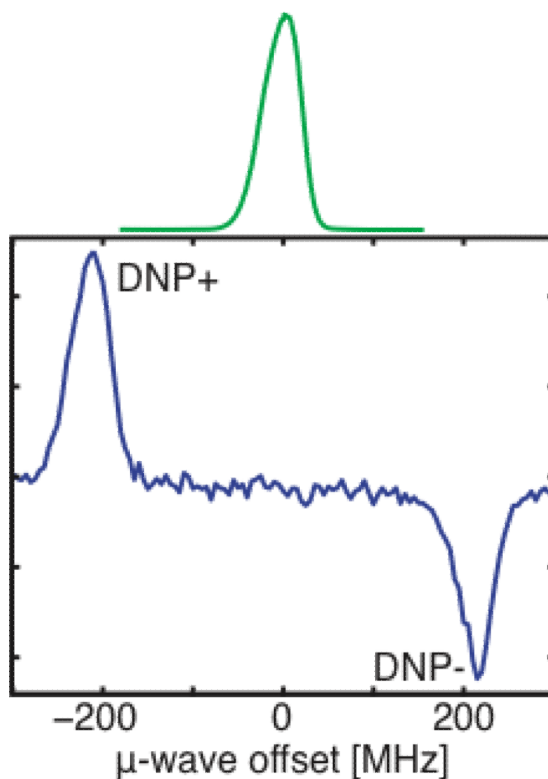
Figure 7. Solid effect DNP Enhancement Profile
